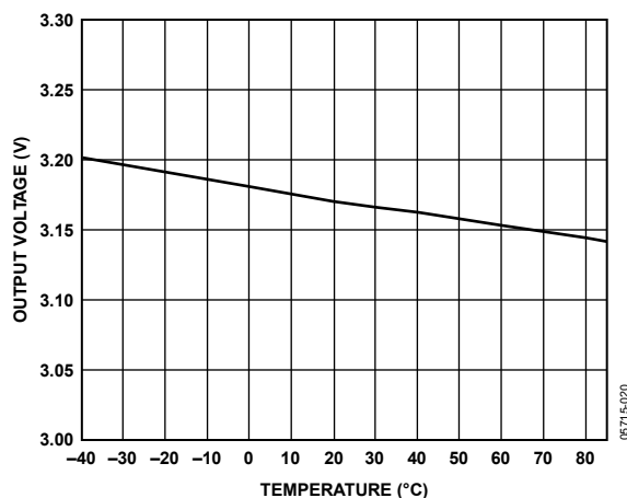
Figure 20. Receiver Output High Voltage vs. Temperature, I_O = 1.5 mA
