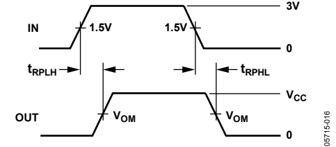
Figure 16. Receiver Propagation Delay
