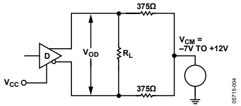
Figure 4. Driver V_{OD} with Varying Common-Mode Voltage
