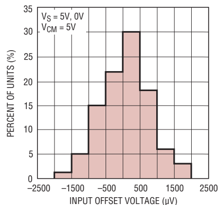
V_{OS} Distribution, V_{CM} = 5\text{V} (SOT-23, NPN Stage)
