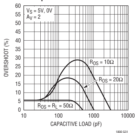
Series Output Resistor vs Capacitive Load
