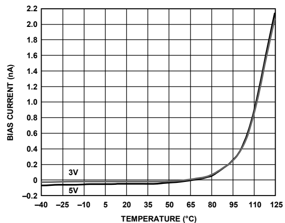
Figure 42. Operational Amplifier Bias Current vs. Temperature
