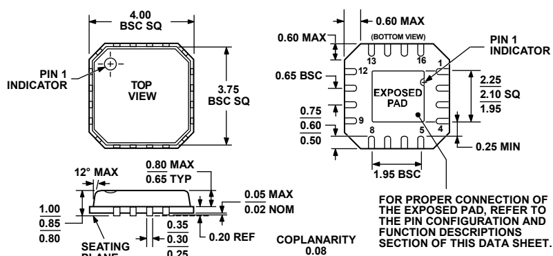
Figure 57. 16-Lead Lead Frame Chip Scale Package [LFCSP_VQ] 4 mm x 4 mm Body, Very Thin Quad (CP-16-4)
