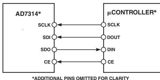
Figure 4. Typical Interface
