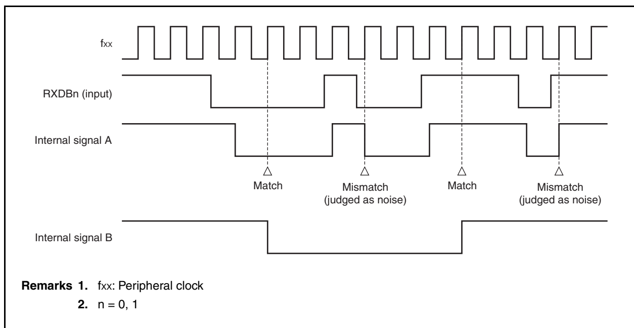
Figure 16-9. Timing of RXDBn Signal Judged as Noise
