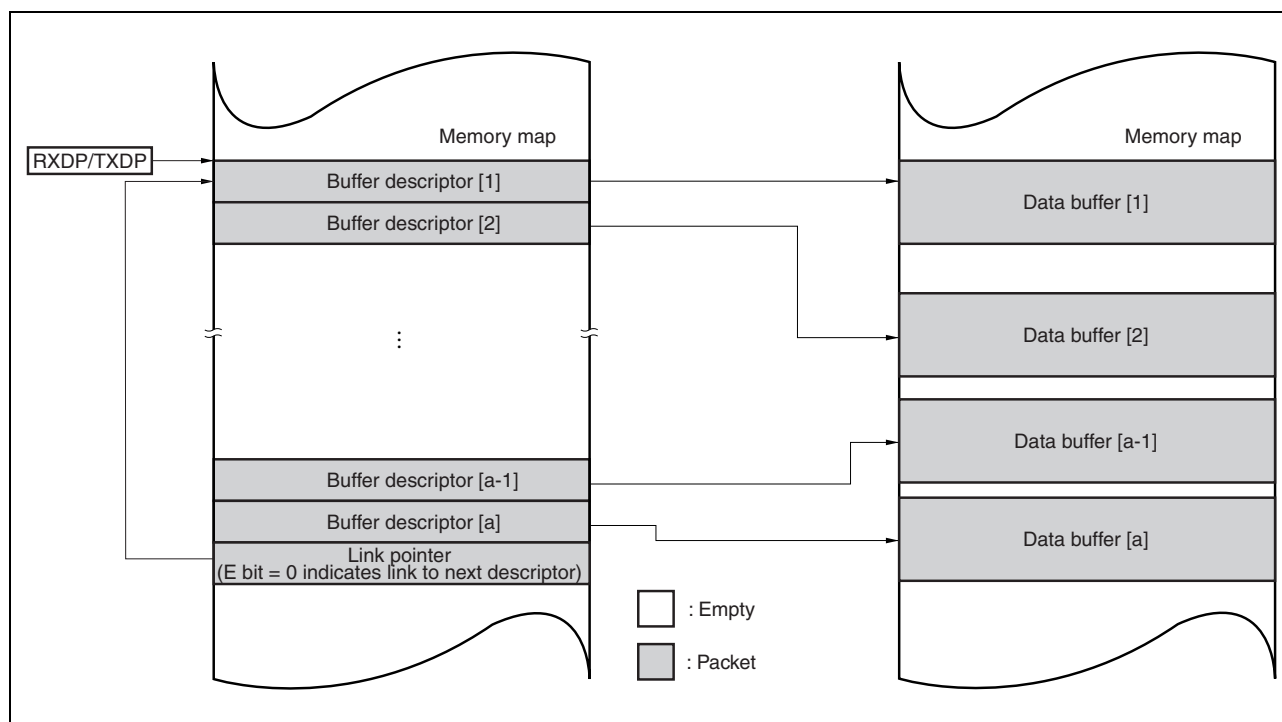
Figure 23-25. Overview of Ring Buffer Formed by Descriptor Chain
