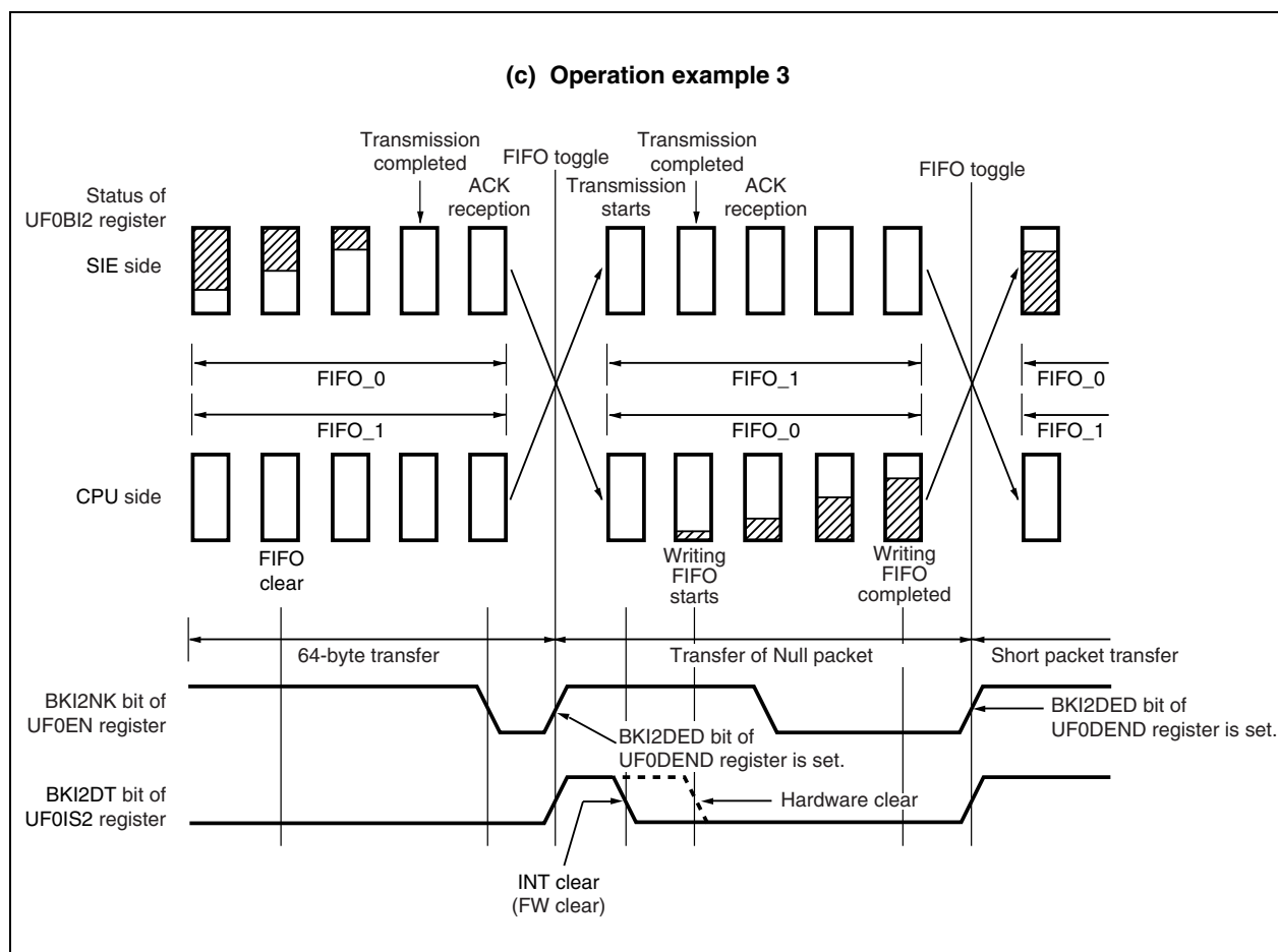
Figure 22-10. Operation of UF0BI2 Register (3/3)
