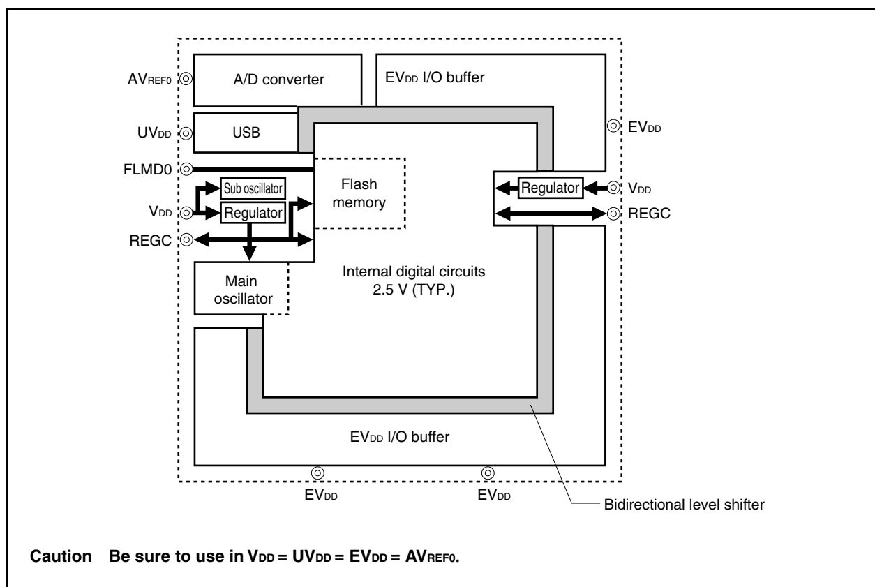
Figure 32-1. Regulator
