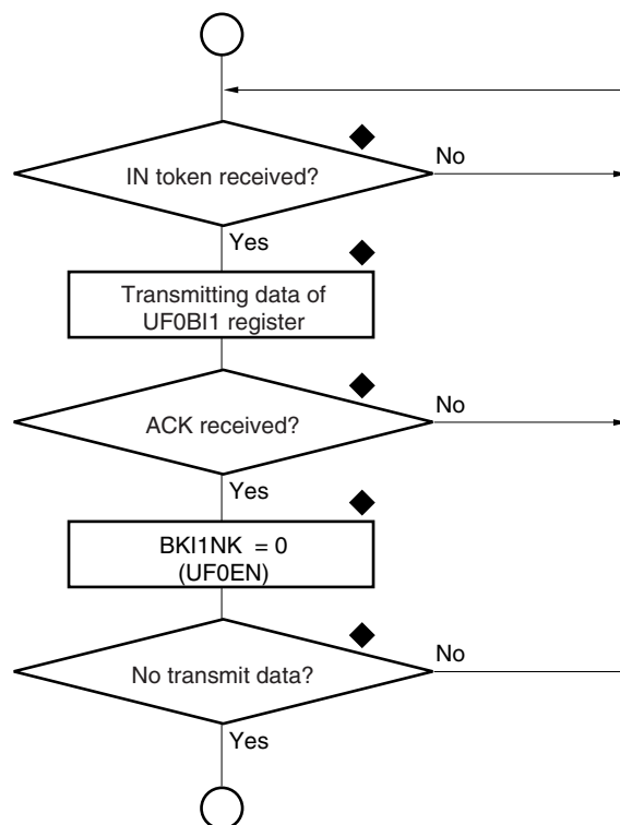
Figure 22-26. Parallel Processing by Hardware
