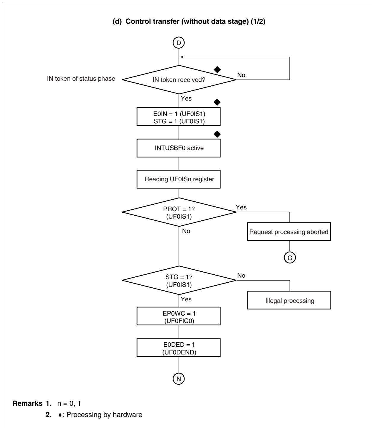
Figure 22-24. CPUDEC Request for Control Transfer (11/12)
