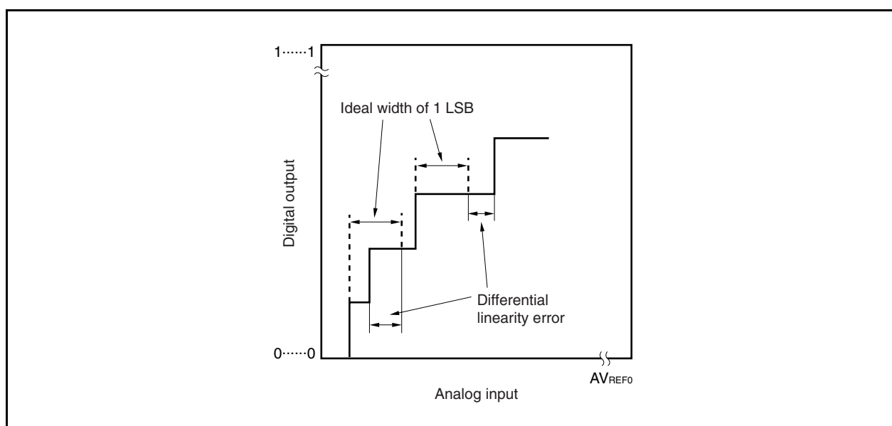
Figure 15-20. Differential Linearity Error
