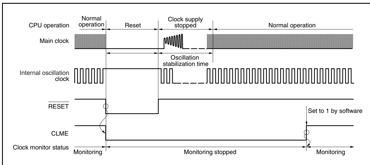
Figure 29-3. Clock Monitor Status After RESET Input
