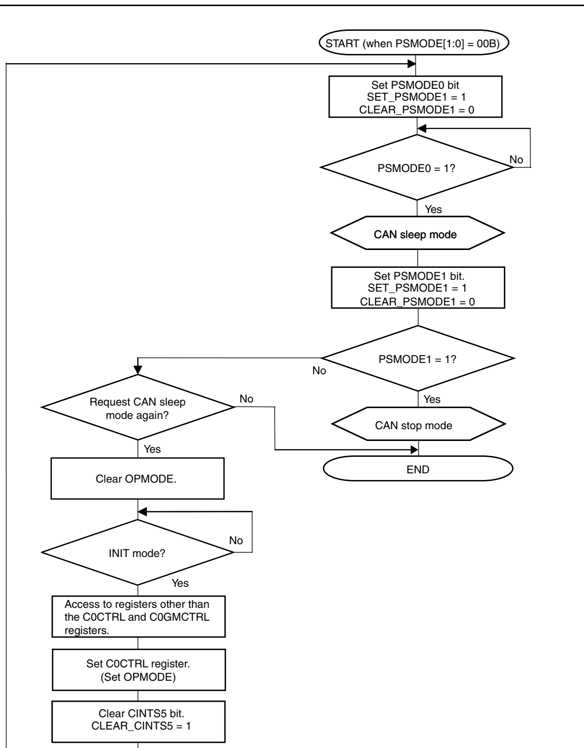
Figure 21-52. Setting CAN Sleep Mode/Stop Mode
