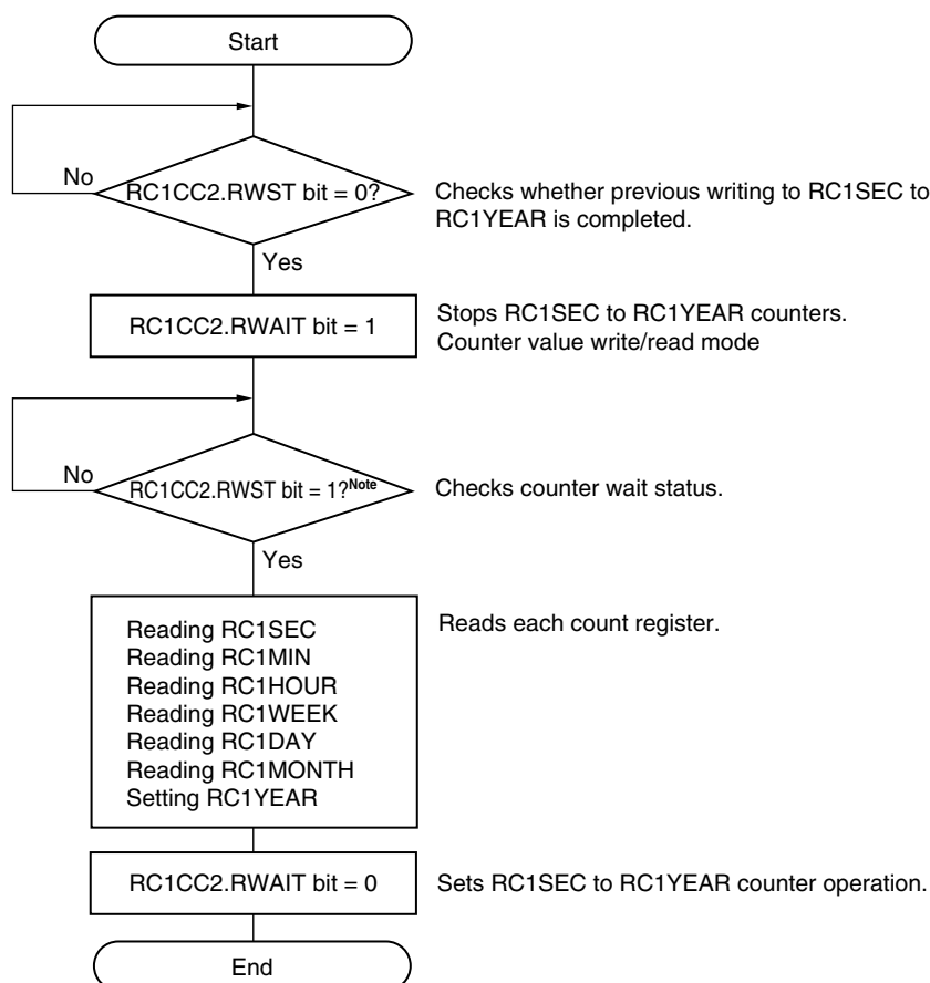
Figure 12-4. Reading Each Counter During Real-time Counter Operation
