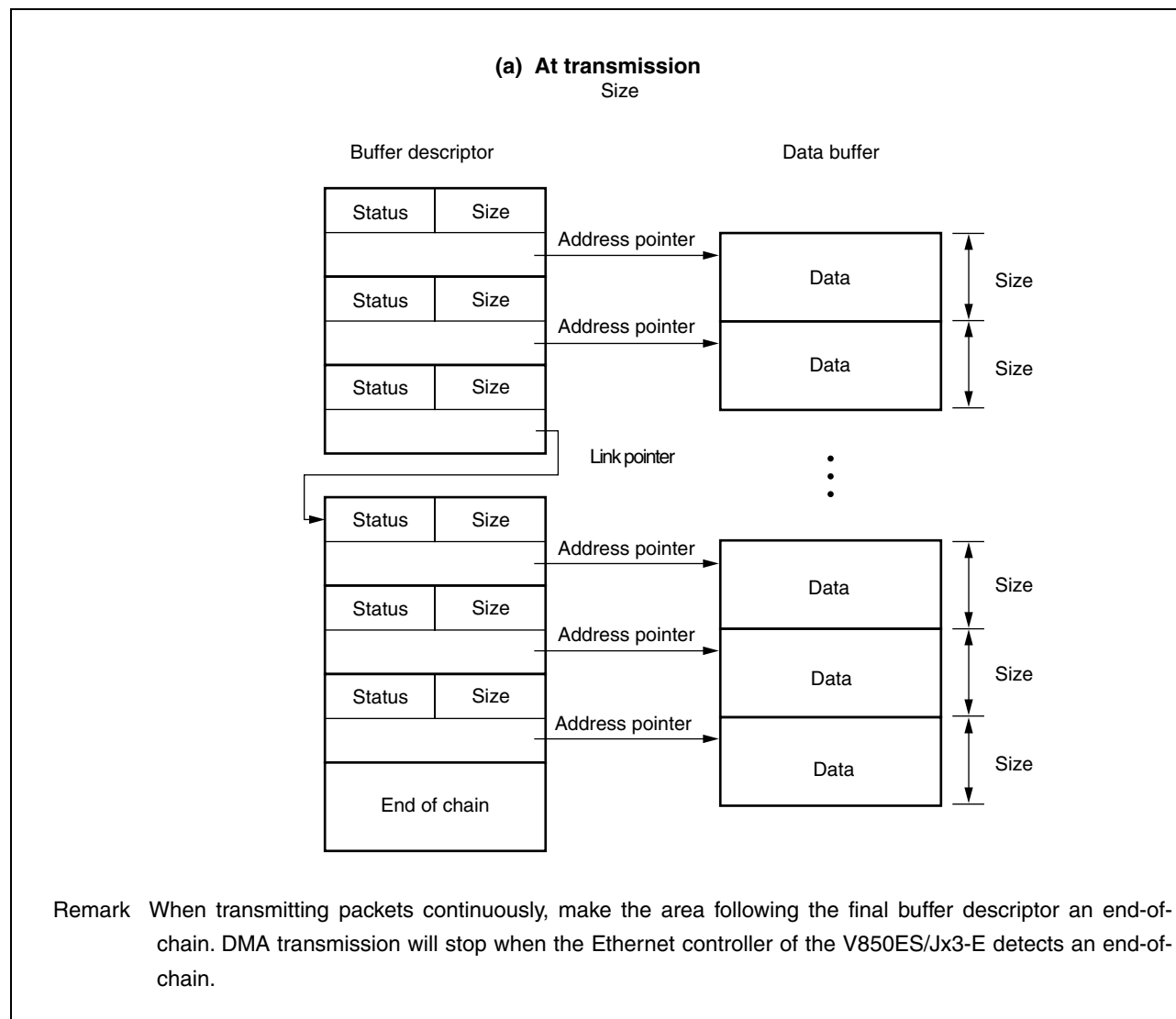
Figure 23-18. Buffer Structure of Ethernet controller(1/2)
