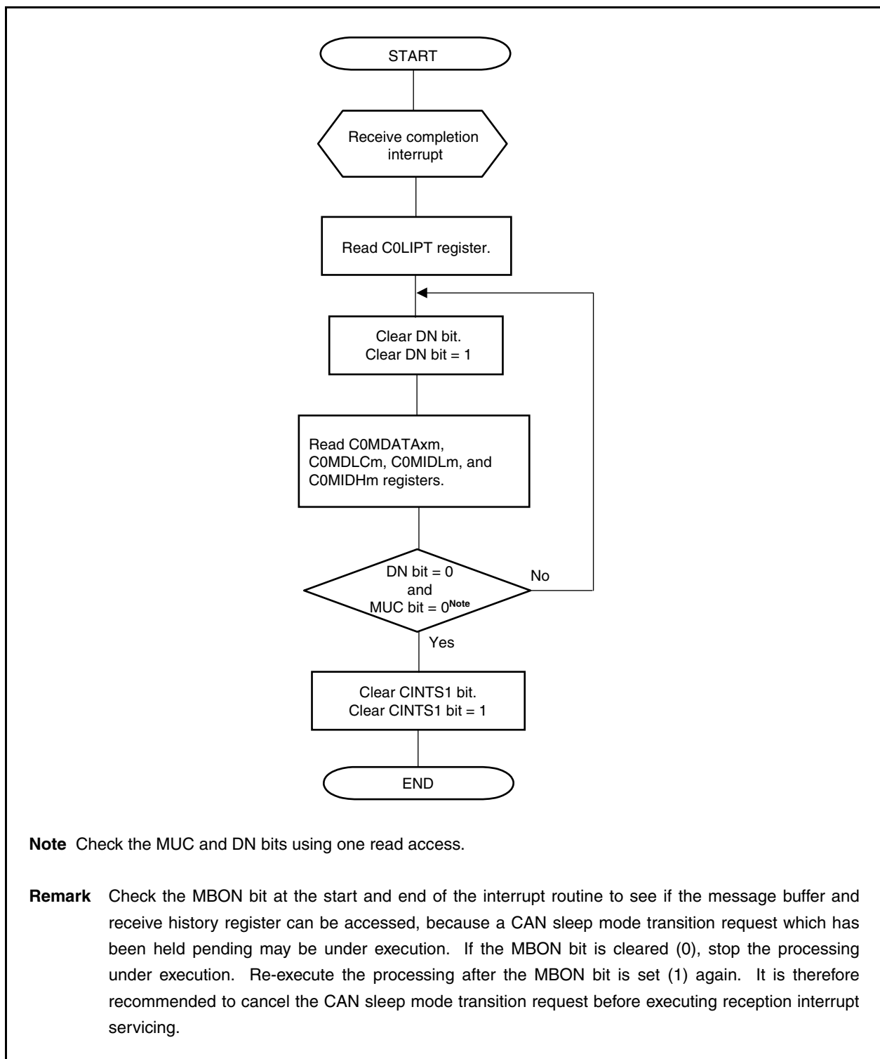
Figure 21-49. Reception via Interrupt (Using C0LIPT Register)
