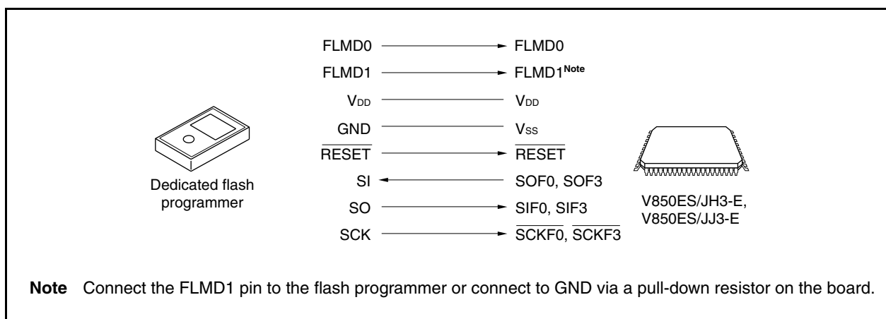
Figure 33-4. Communication with Dedicated Flash Programmer (CSIF0, CSIF3)
