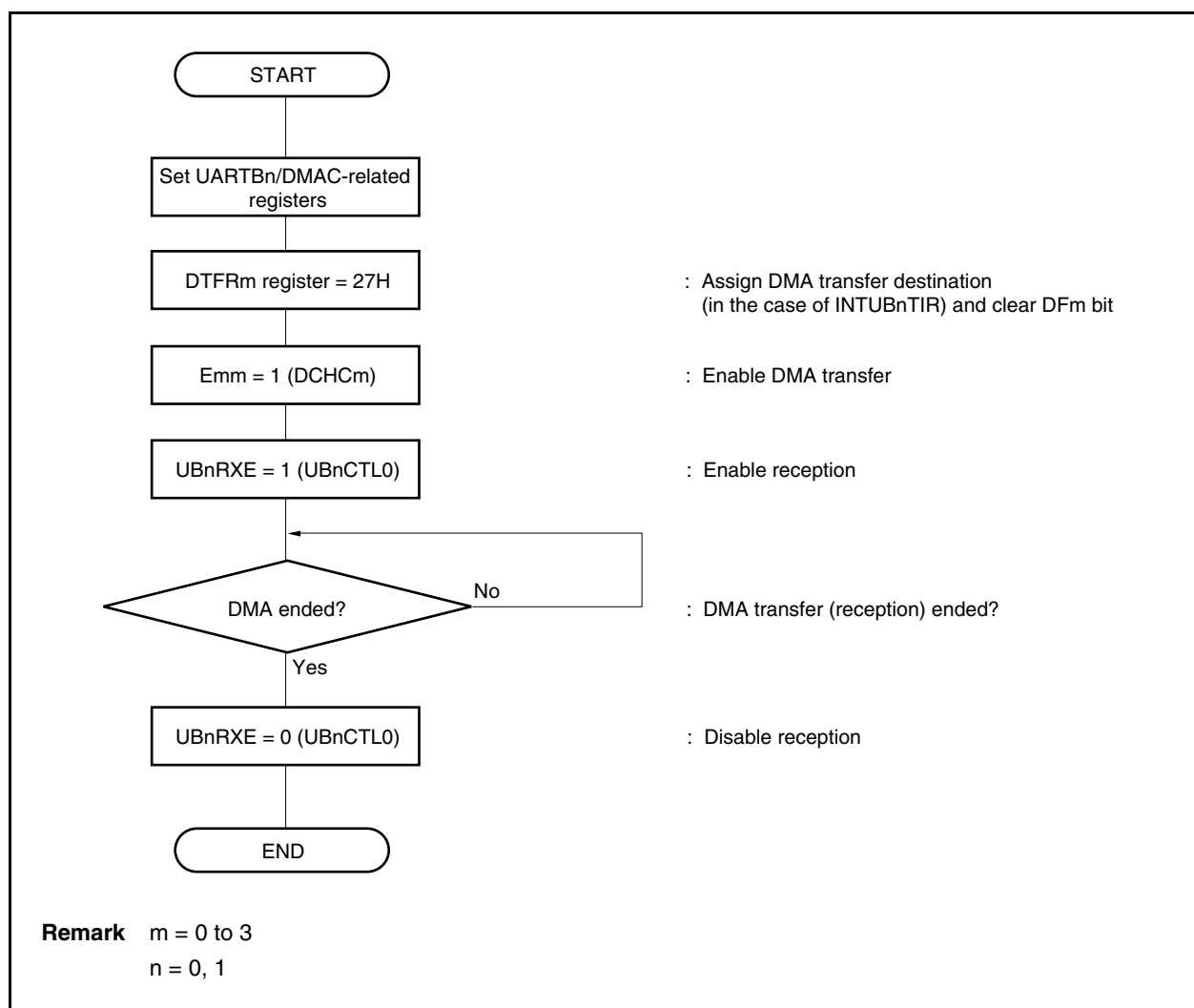
Figure 16-16. Example of Continuous Reception Processing Flow in Single Mode (DMA Control)
