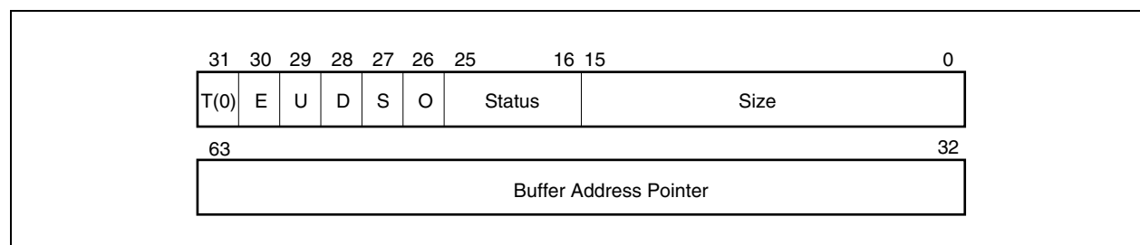
Figure 23-19. Buffer Descriptor Format
