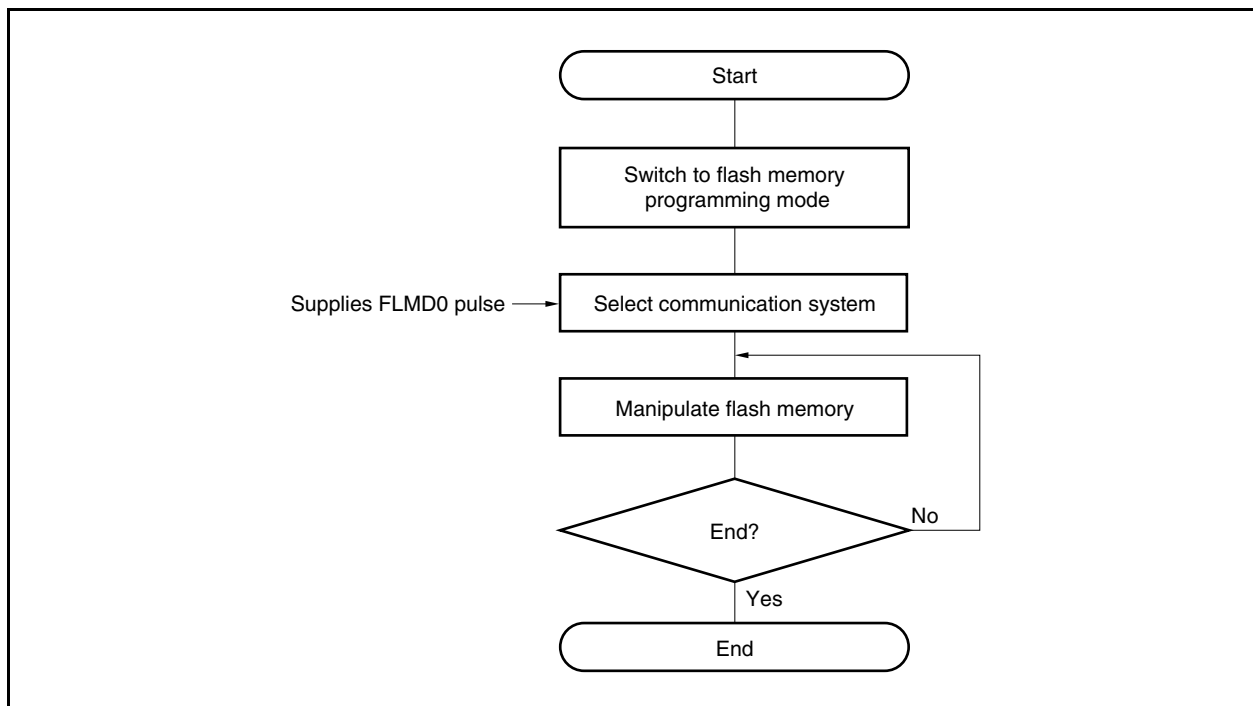
Figure 33-8. Procedure for Manipulating Flash Memory
