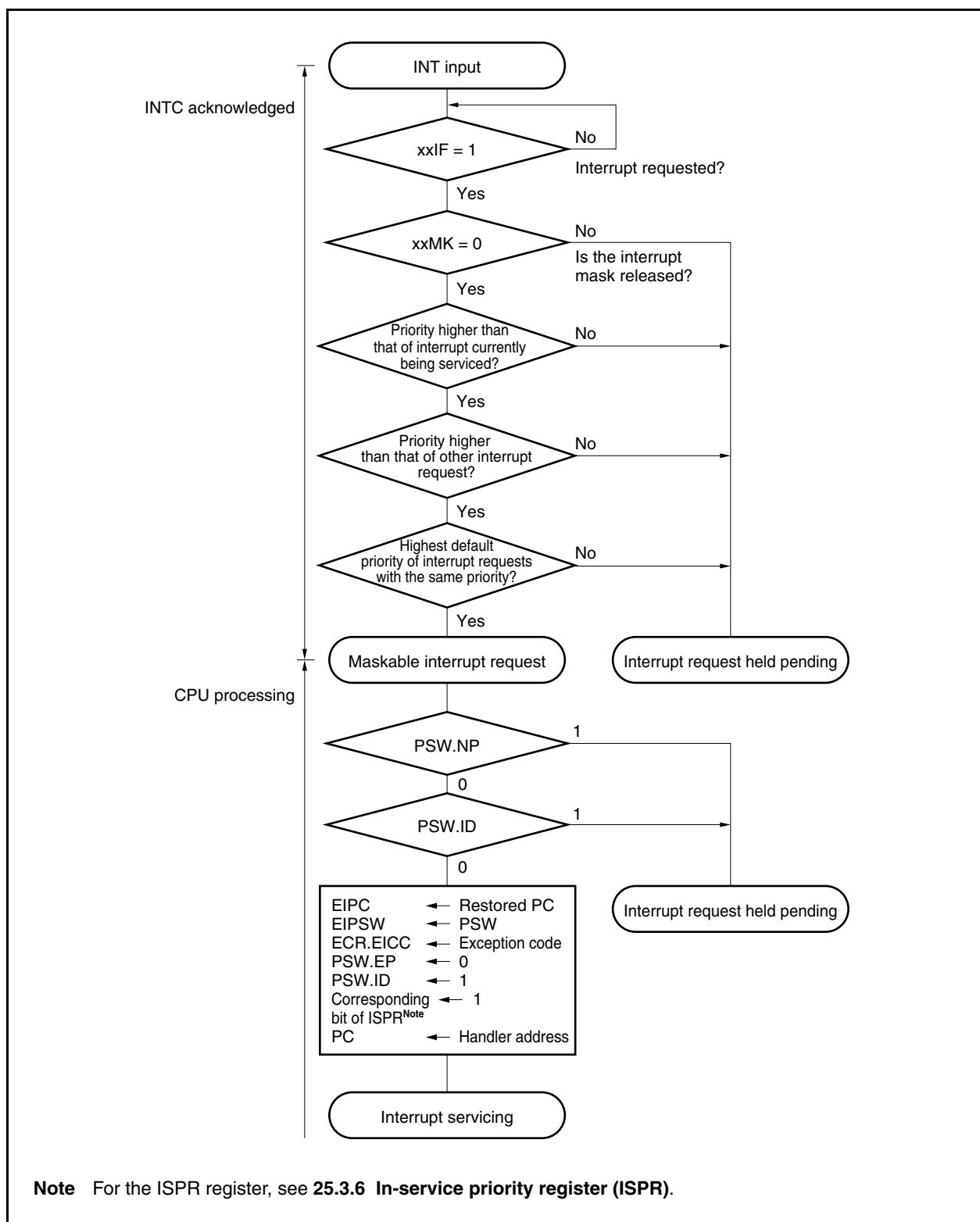
Figure 25-5. Maskable Interrupt Servicing
