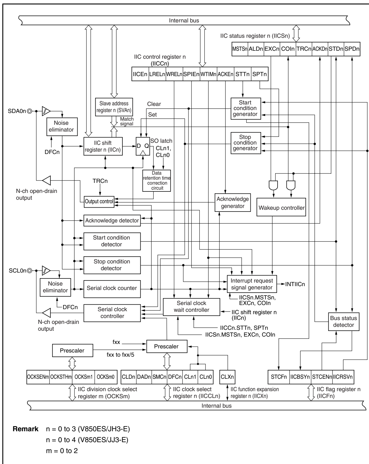
Figure 20-1. Block Diagram of I 2 C0n
