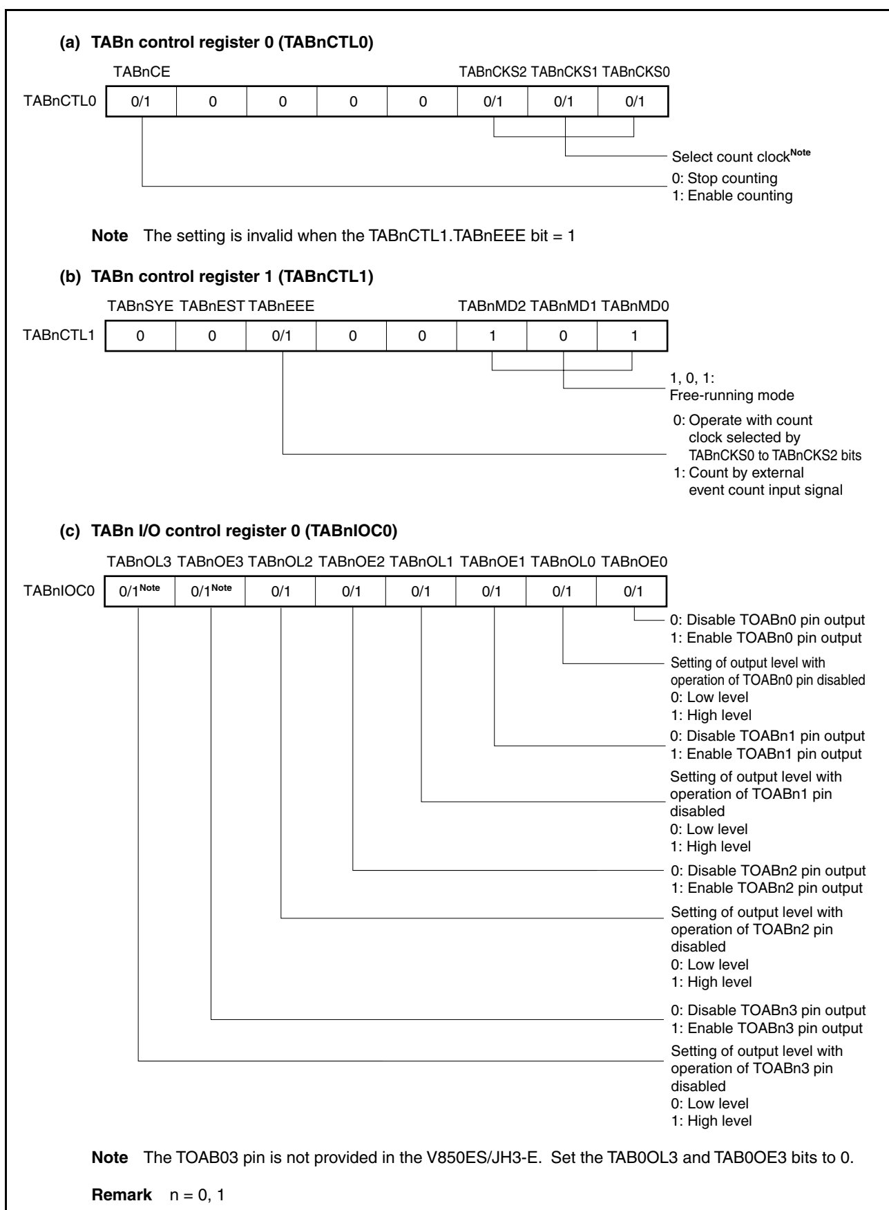
Figure 8-31. Register Setting in Free-Running Timer Mode (1/3)
