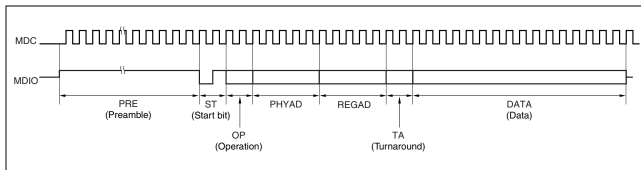
Figure 23-12. Serial Management Frame Structure
