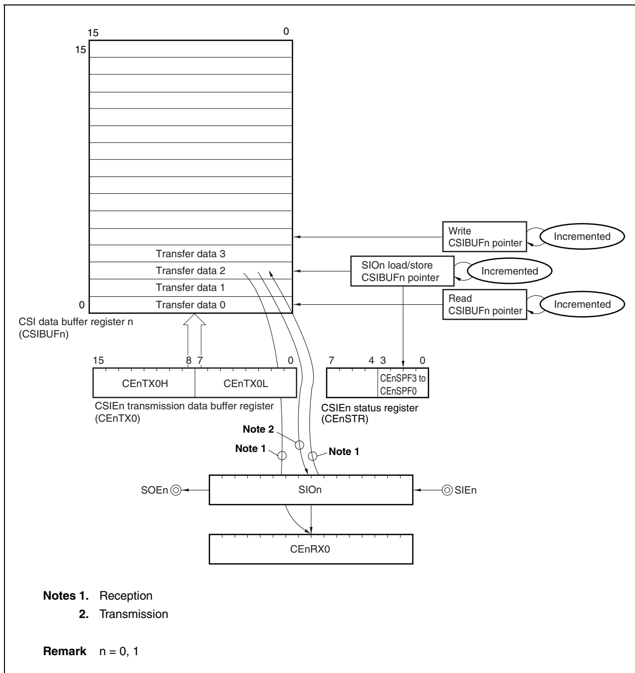
Figure 18-11. Continuous Mode
