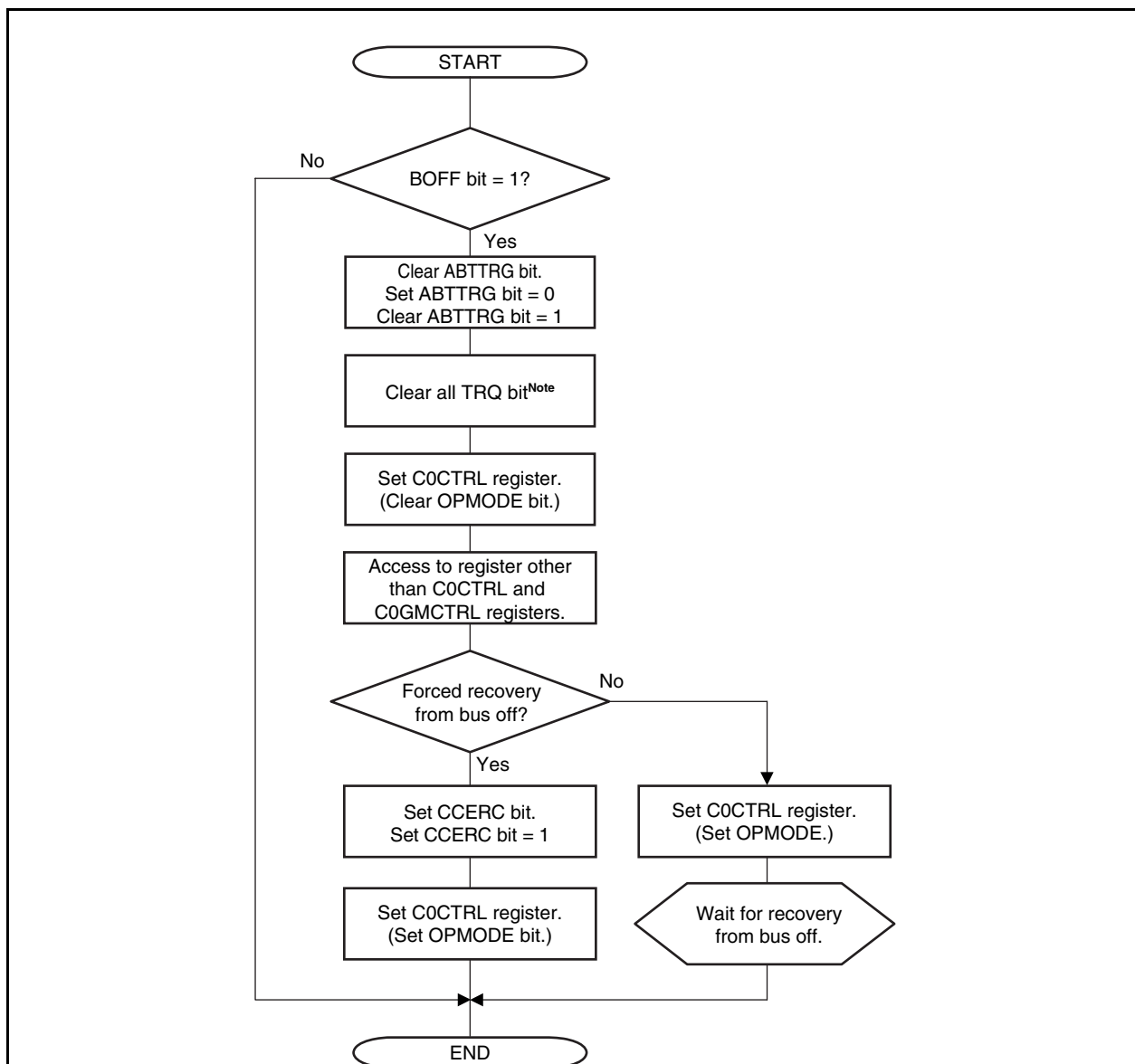
Figure 21-55. Bus-off Recovery (Normal Operation Mode with ABT)
