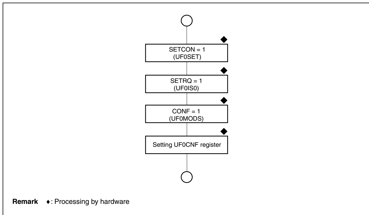
Figure 22-23. SET_INTERFACE Processing
