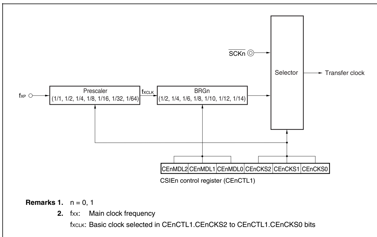
Figure 18-2. Transfer Clock of CSIE n
