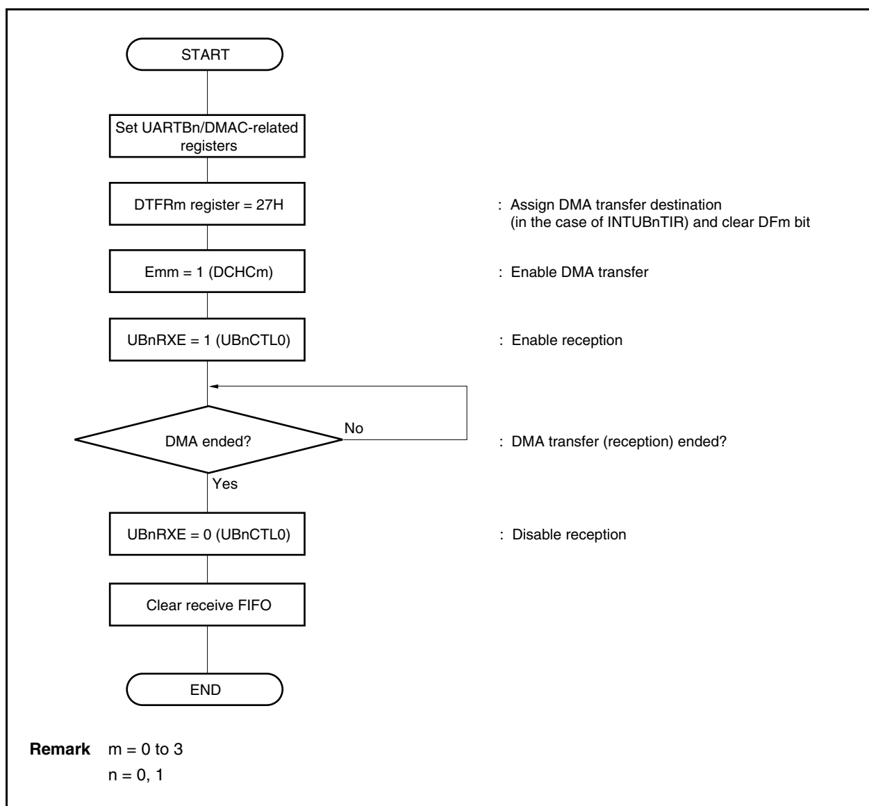
Figure 16-20. Example of Continuous Reception (Pending Mode) Processing Flow in FIFO Mode (DMA Control)
