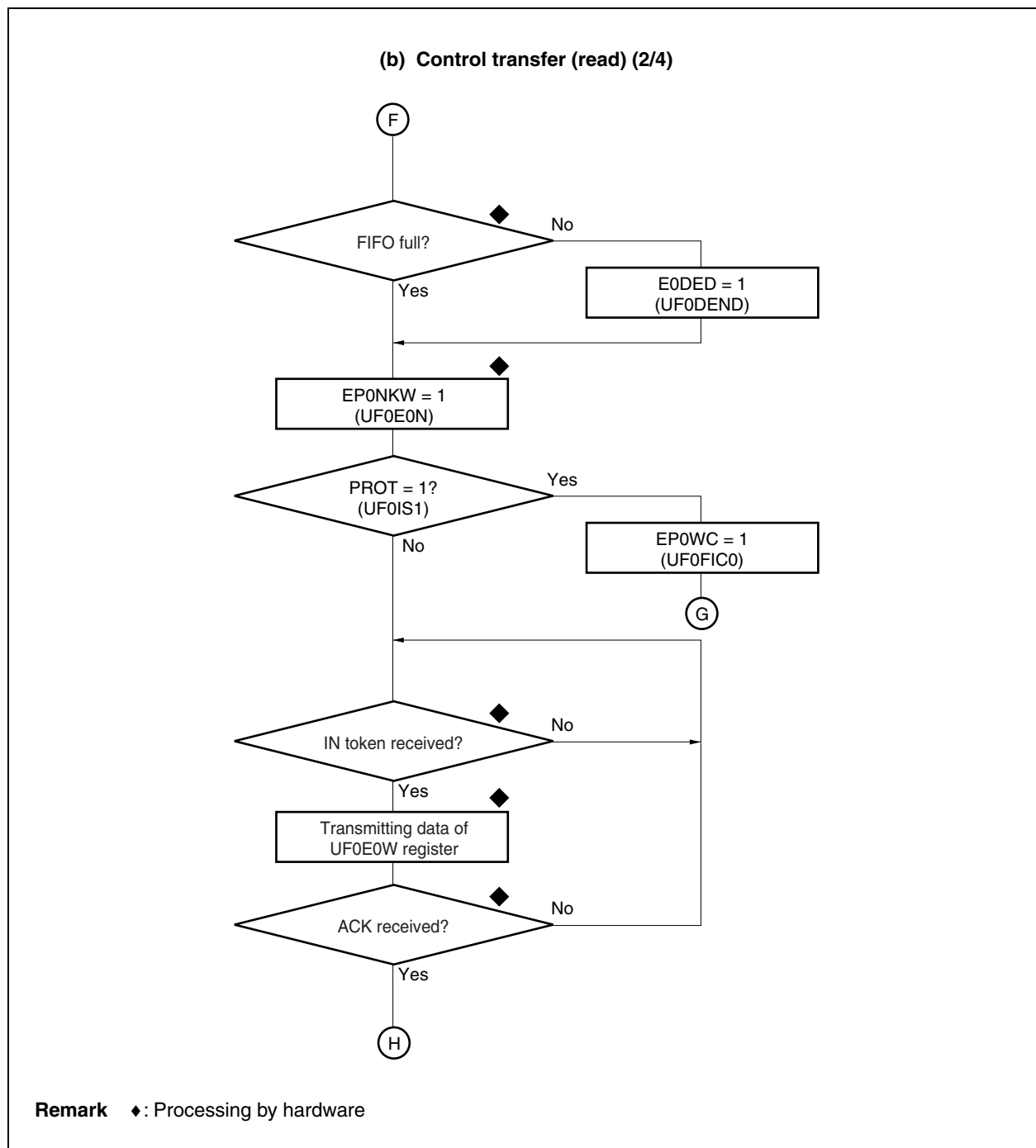
Figure 22-24 CPUDEC Request for Control Transfer (4/12)
