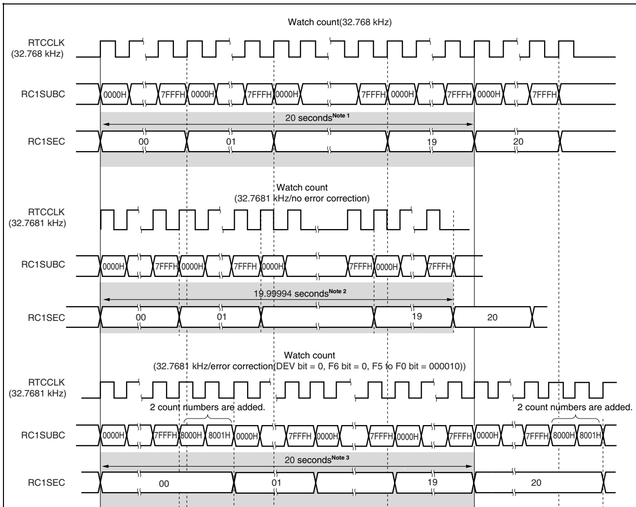
Figure 12-10. Watch Error Correction Example
