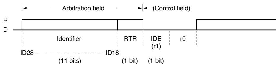
Figure 21-6. Arbitration Field (in Standard Format Mode)
