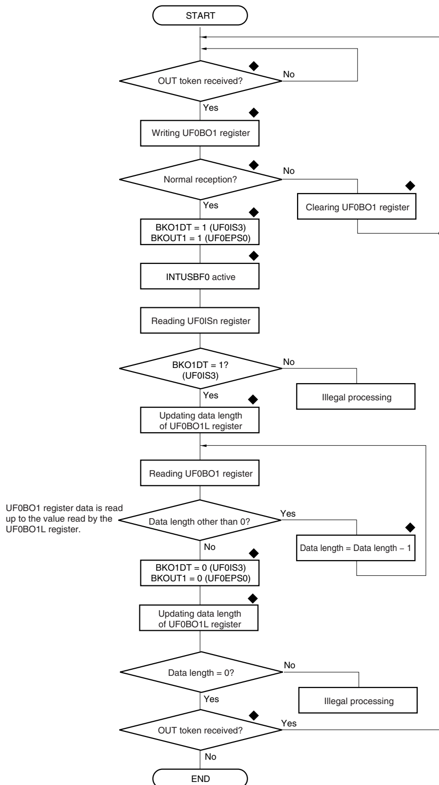
Figure 22-27. Normal Processing for Bulk Transfer (OUT) (Endpoint2)
