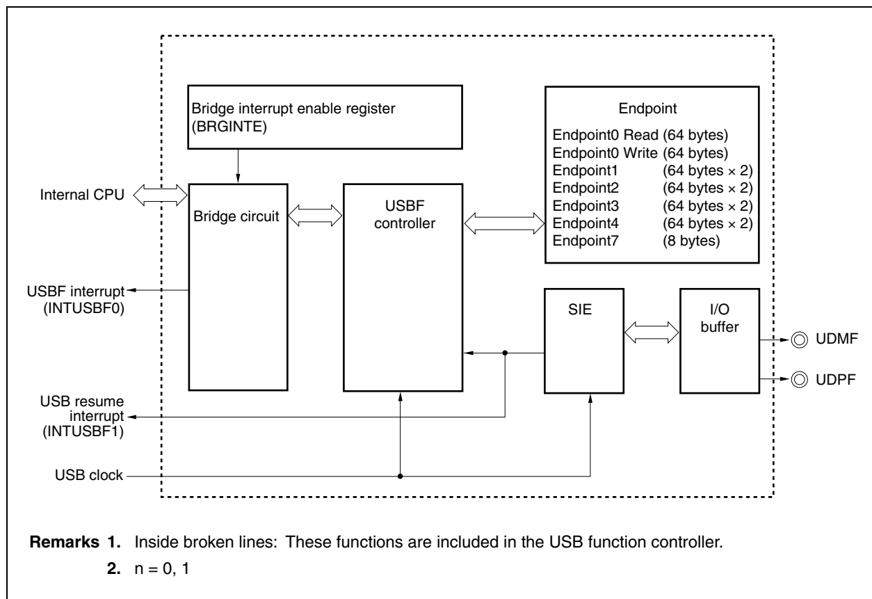
Figure 22-1. Block Diagram of USB Function Controller
