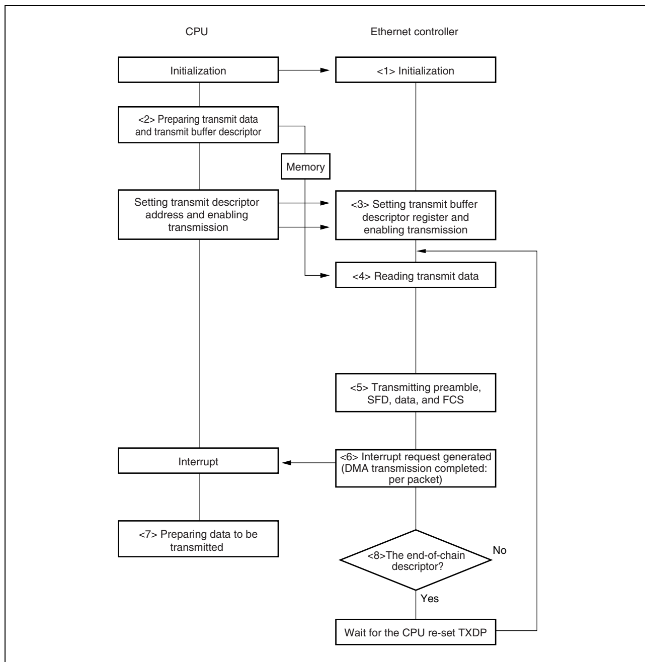
Figure 23-26. Example of Ethernet Transmission Procedure
