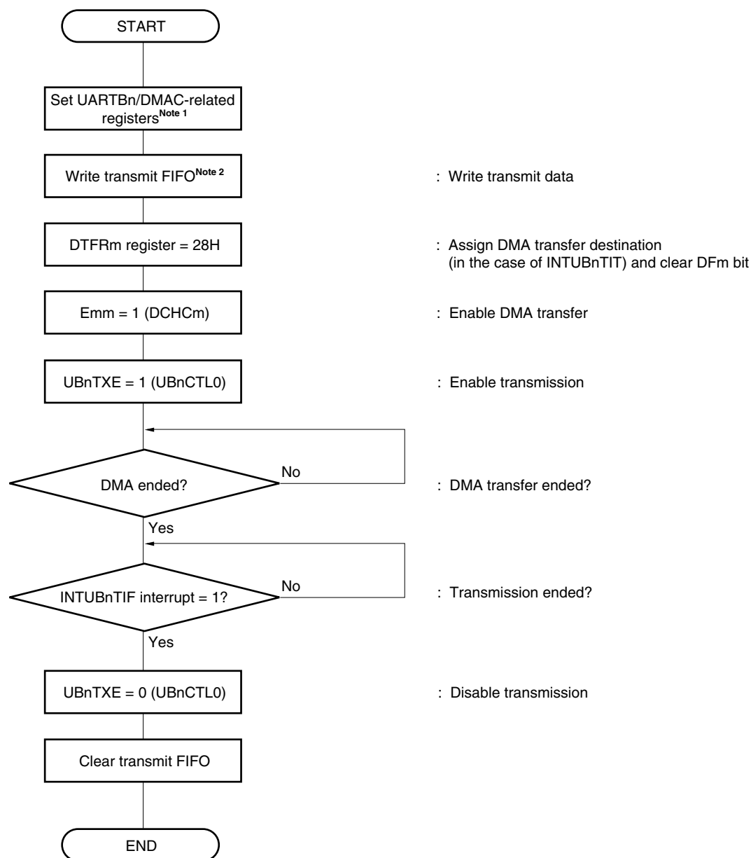
Figure 16-19. Example of Continuous Transmission (Pending Mode) Processing in FIFO Mode (DMA Control)
