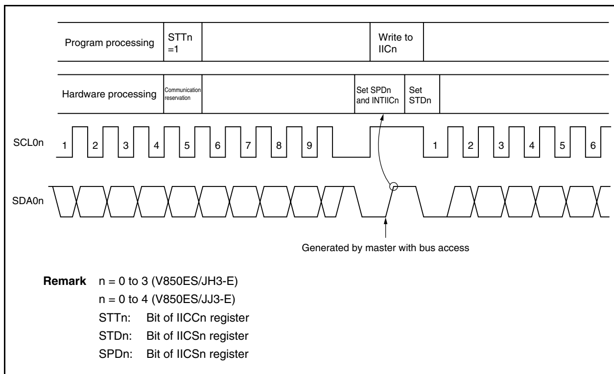
Figure 20-16. Communication Reservation Timing
