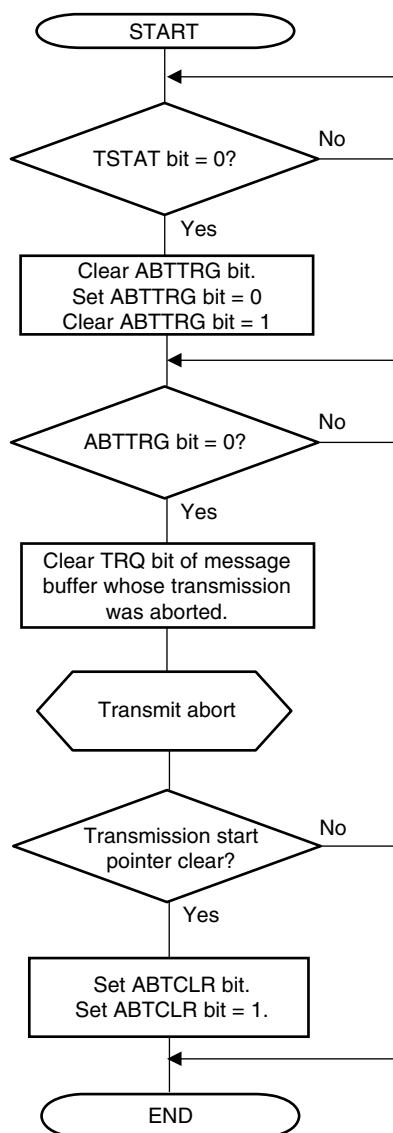
Figure 21-48 (a). ABT Transmission Abort Processing (Normal Operation Mode with ABT)
