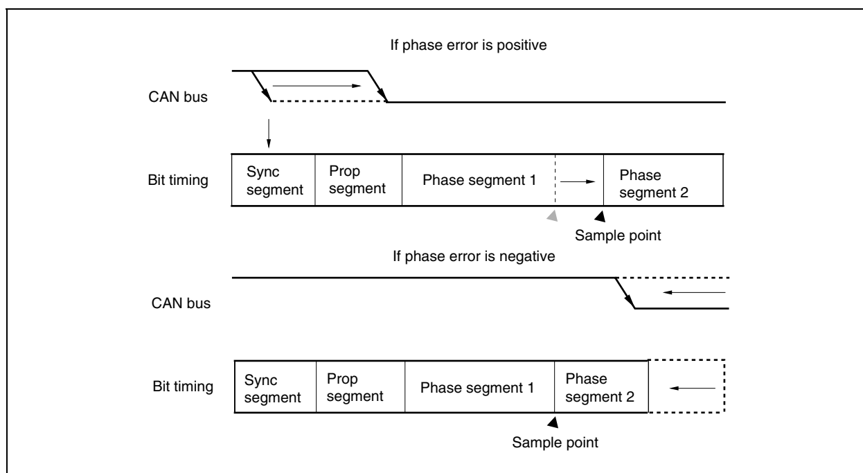
Figure 21-21. Resynchronization
