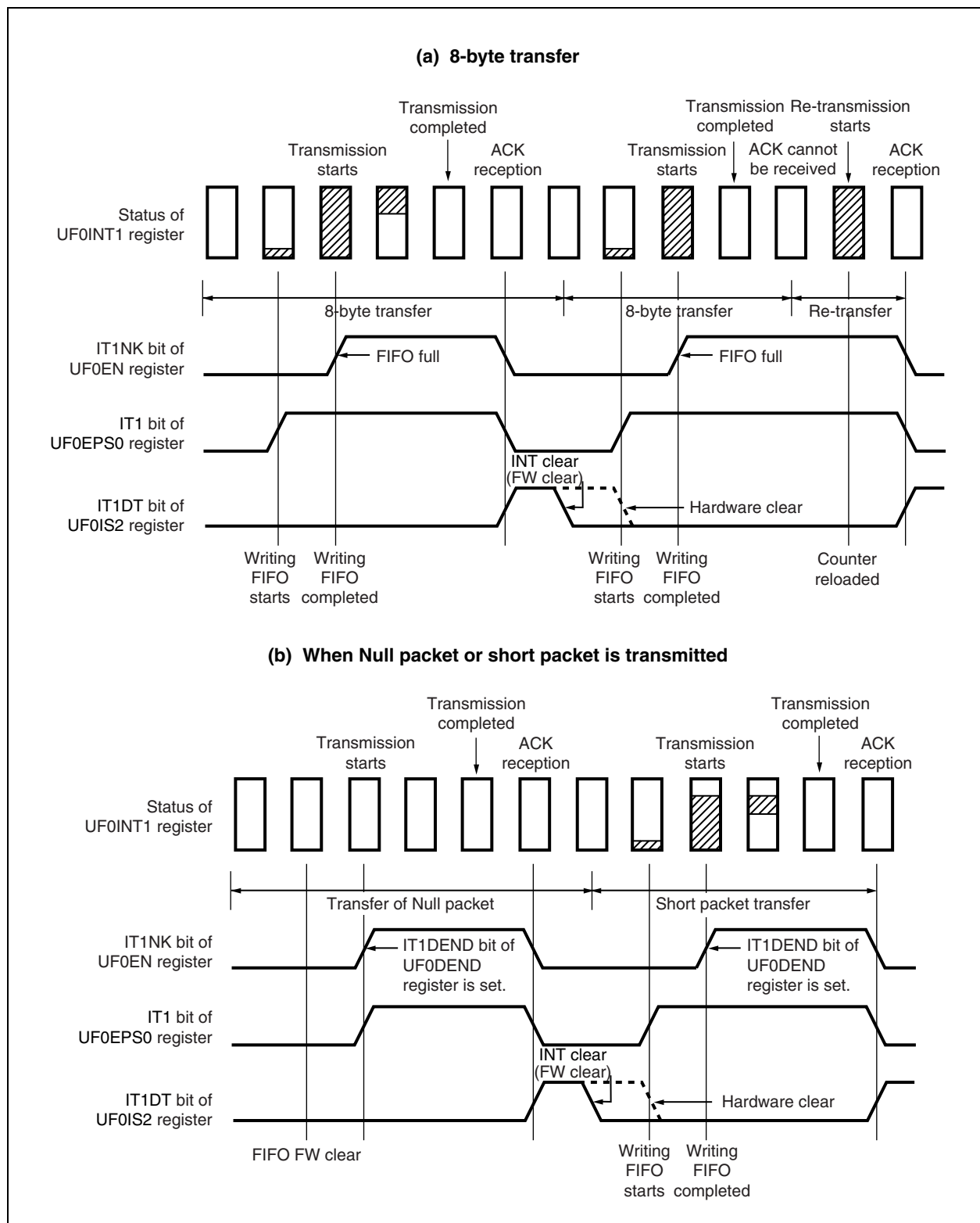
Figure 22-11. Operation of UF0INT1 Register
