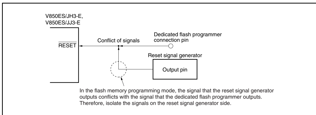
Figure 33-15. Conflict of Signals (RESET Pin)
