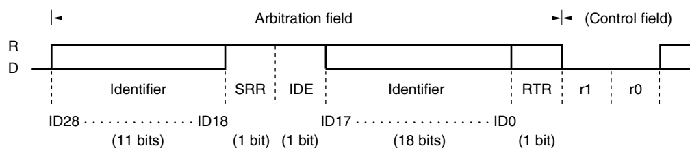
Figure 21-7. Arbitration Field (in Extended Format Mode)
