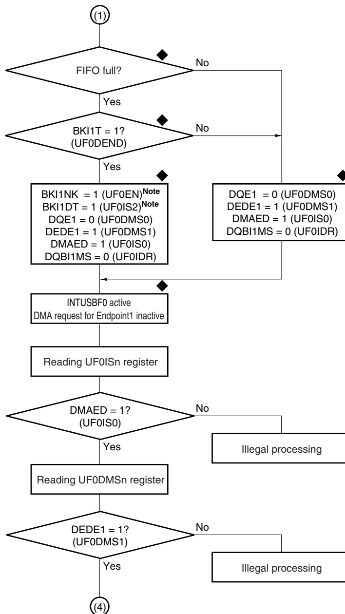
Figure 22-33. DMA Processing by Bulk Transfer (IN) (3/4)
