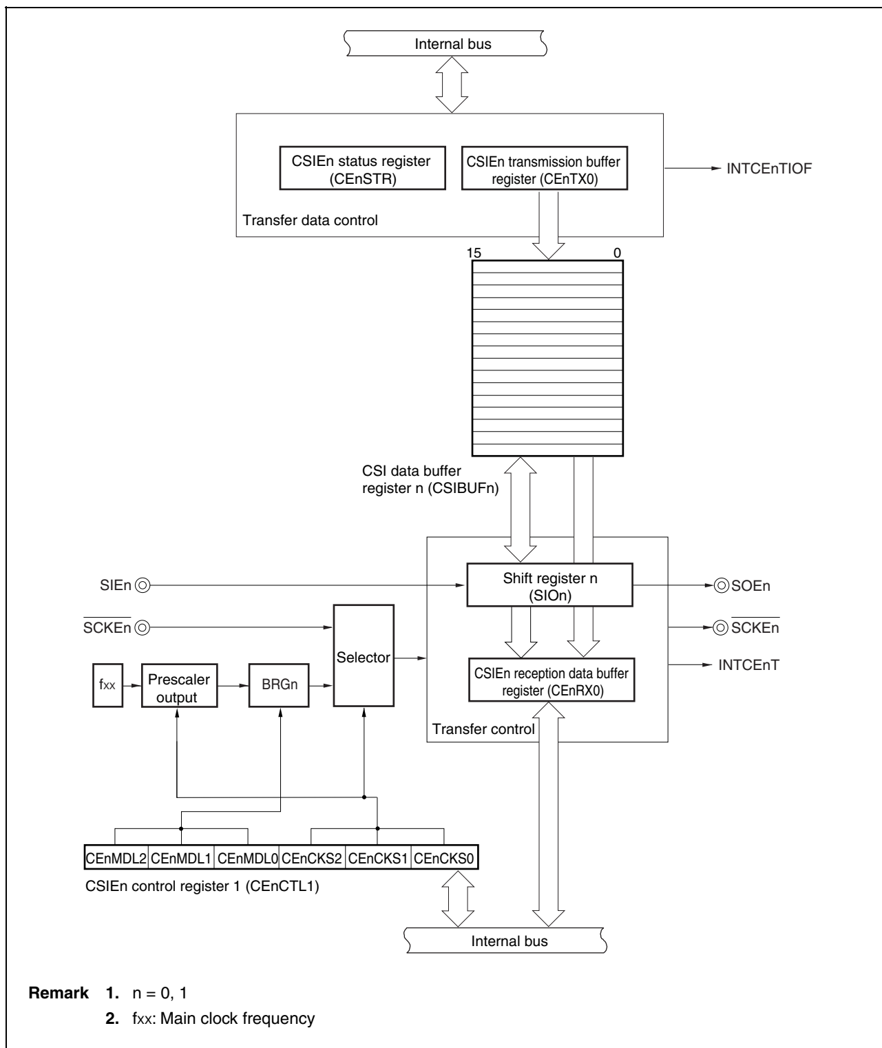
Figure 18-1. Block Diagram of CSIE n
