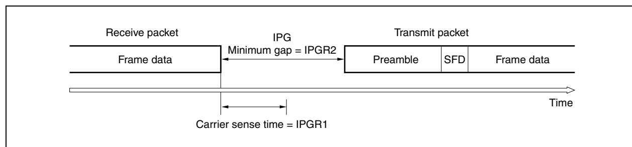
Figure 23-7. IPG During Non Back-To-Back Transmission
