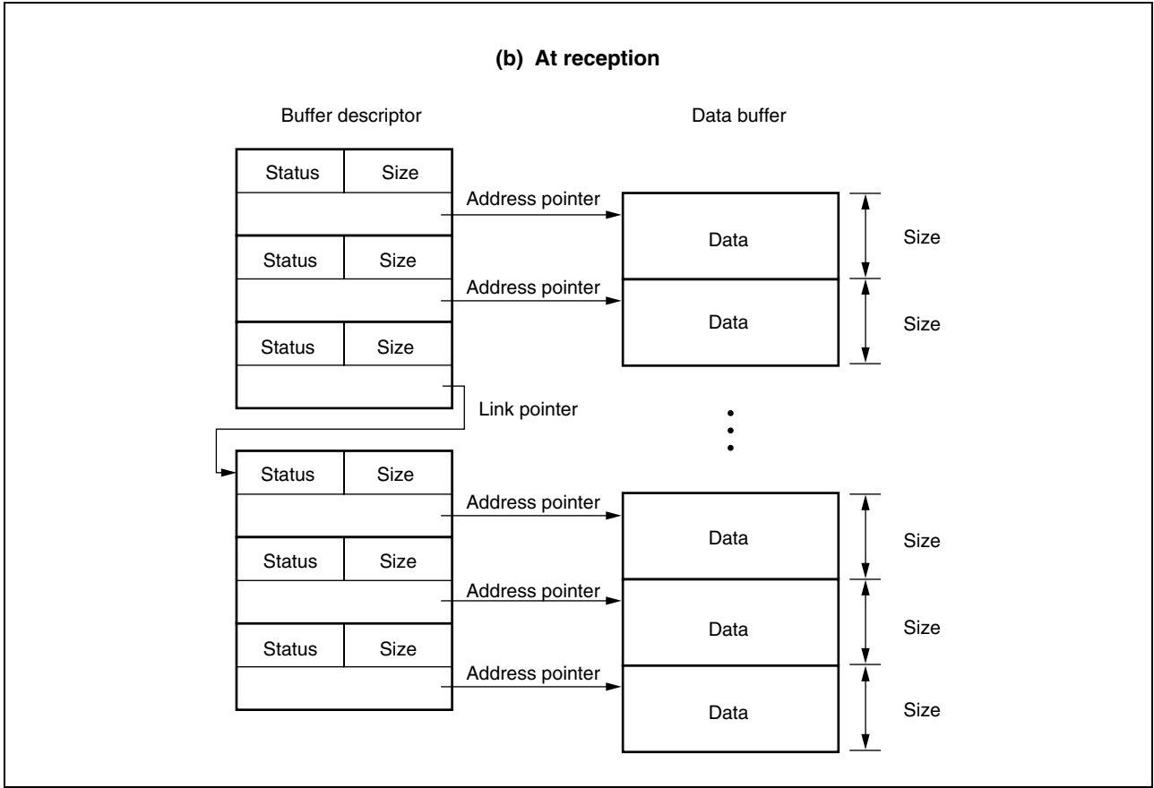
Figure 23-18. Buffer Structure of Ethernet controller(2/2)
