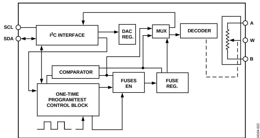
Figure 33. Detailed Functional Block Diagram
