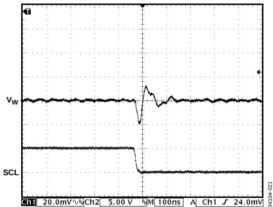
Figure 23. Digital Feedthrough
