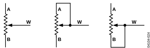
Figure 34. Rheostat Mode Configuration
