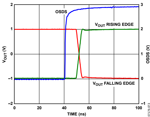
Figure 76. ADV3201 OSD Switching Time
