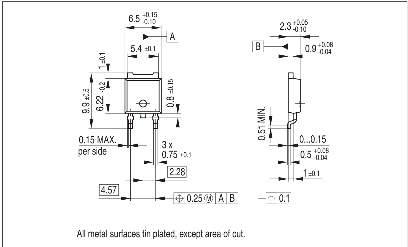
Figure 4 PG-TO-252-3 (Plastic Small Outline Transistor)
