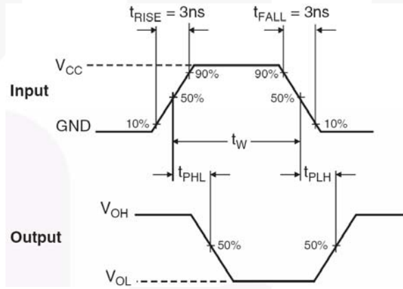
Figure 6. AC Waveforms
