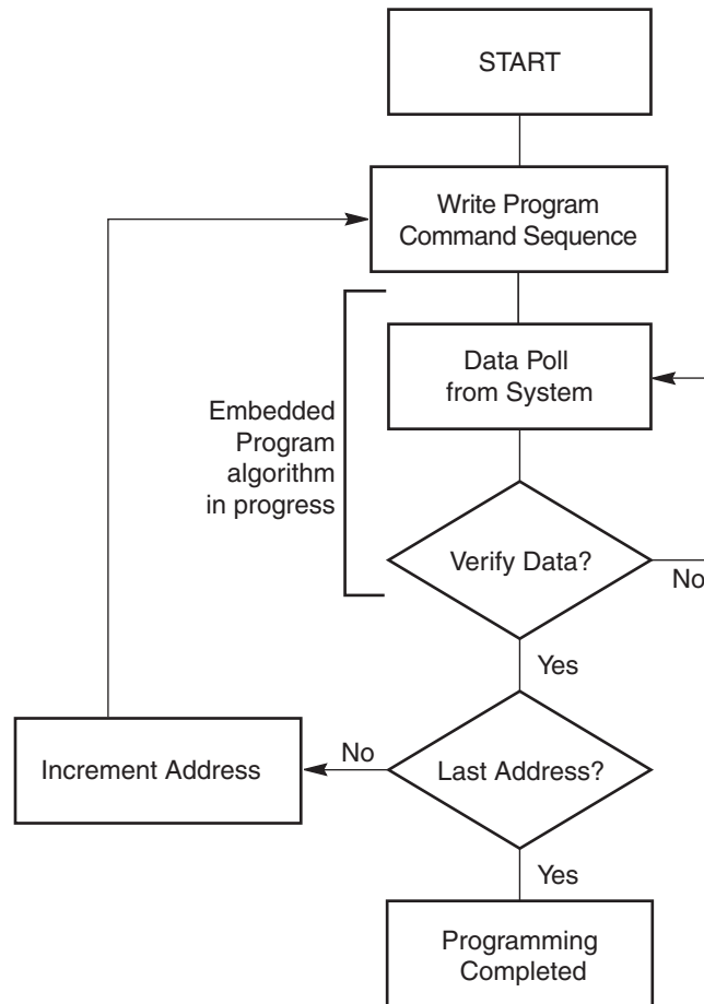
Figure 11.1 Program Operation
