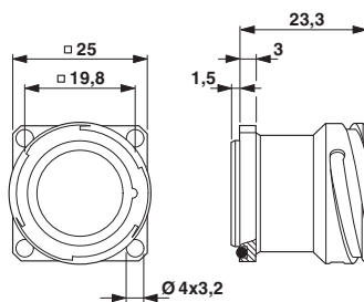
Dimensioned drawing
