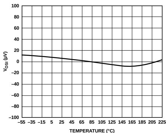
Figure 2. Typical Input Offset vs. Temperature ( G = 100 )
