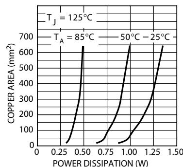
Figure 5. Copper Area vs. Power-SOIC Power Dissipation
