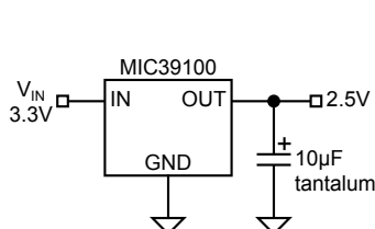
2.5V/1A Regulator
