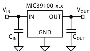
Figure 1. Capacitor Requirements
