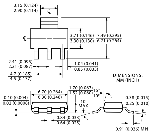
SOT-223 (S)
