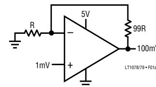
Figure 1b. Voltage Follower
