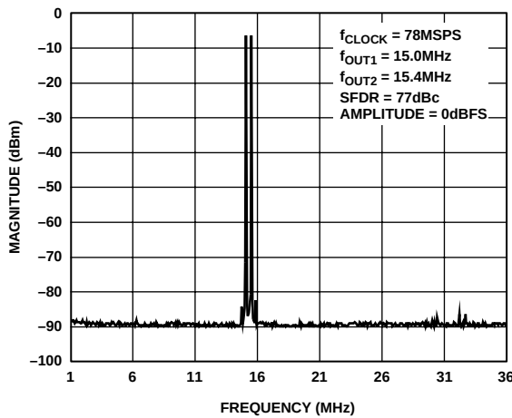
Figure 20. Dual-Tone SFDR
