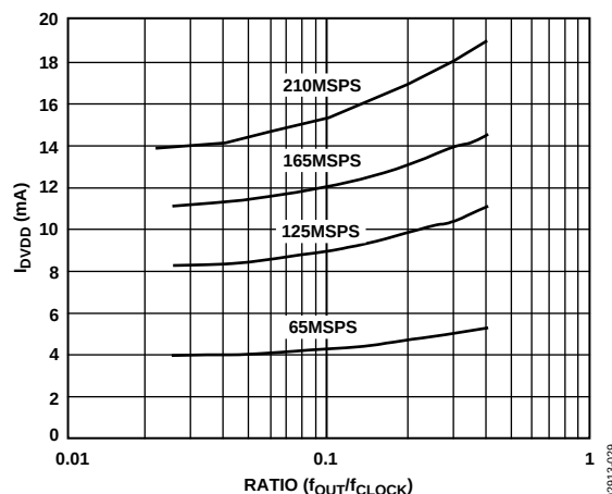
Figure 32. I_{DVDD} vs. Ratio @ DVDD = 3.3 V
