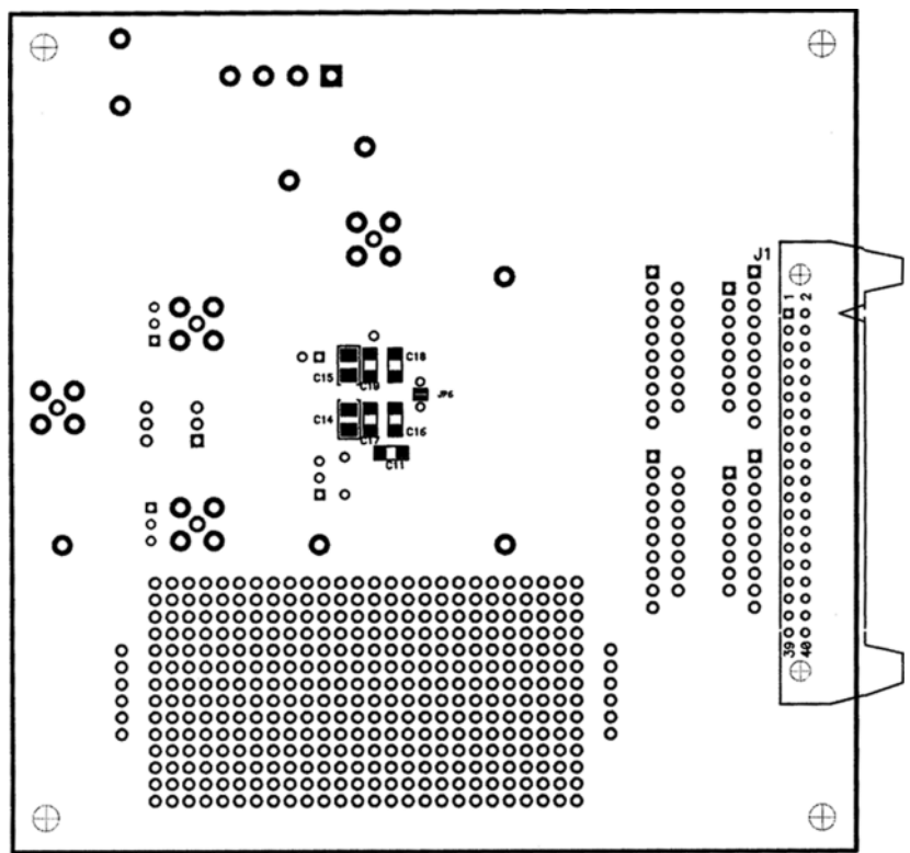
Figure 48. SOIC Evaluation Board Assembly—Secondary Side
