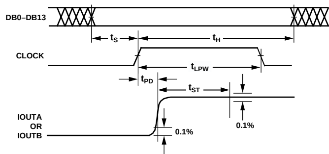
Figure 2. Timing Diagram
