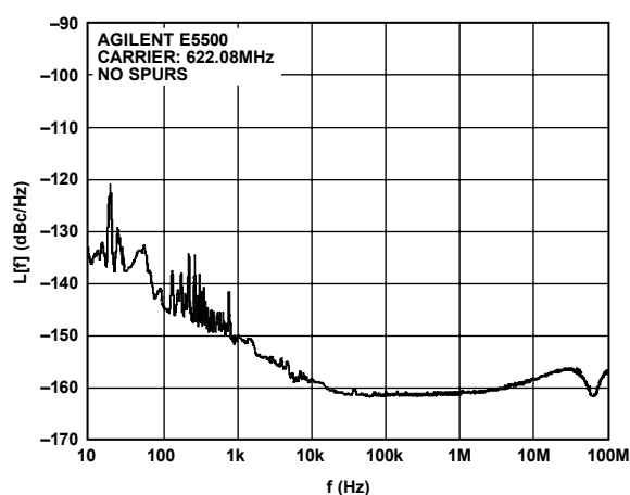
Figure 11. Phase Noise at 622.08 MHz
