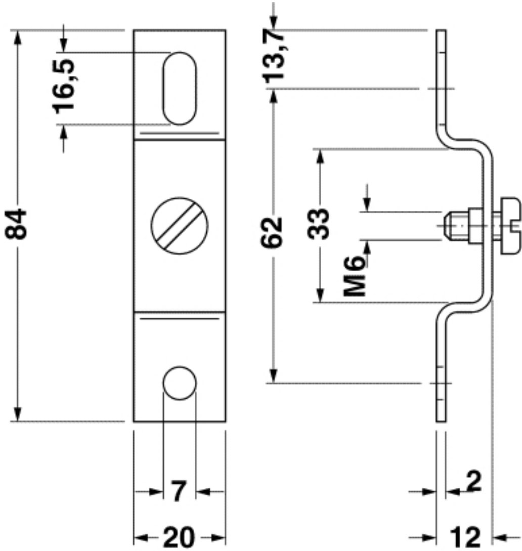
Dimensioned drawing
