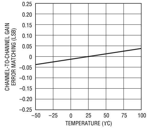
LTC1854 Channel-to-Channel Gain Error Matching vs Temperature
