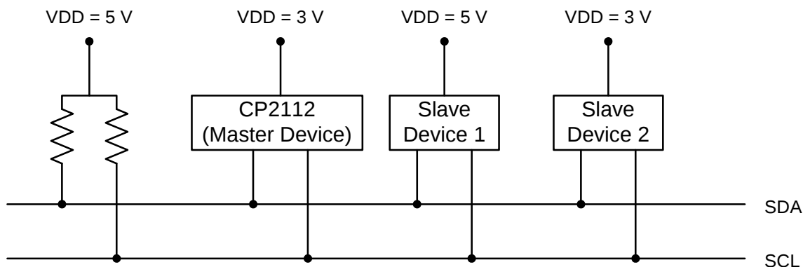
Figure 5. Typical SMBus Configuration
