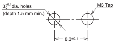
Mounting Hole Dimensions (Reference)
