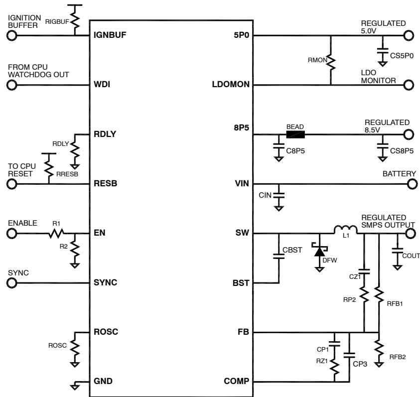
Figure 1. Typical Application
