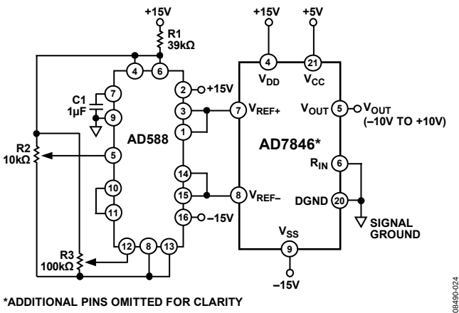
Figure 24. Bipolar ±10 V Operation
