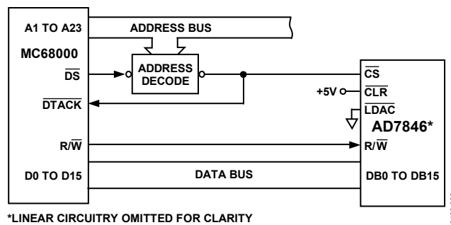
Figure 28. AD7846-to-MC68000 Interface
