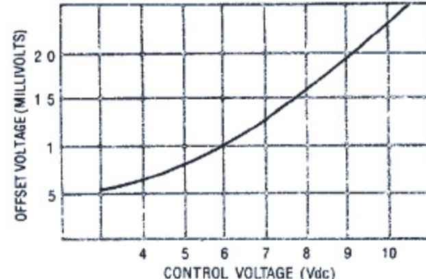
FIGURE 3 - OFFSET VOLTAGE VS. INPUT CONTROL VOLTAGE (TYPICAL)
