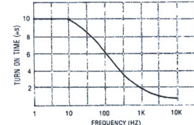
FIGURE 8 - TURN ON TIME VS. DRIVE FREQUENCY (TYPICAL)
