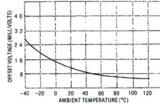
FIGURE 6 - OFFSET VOLTAGE VS. AMBIENT TEMPERATURE (TYPICAL)
