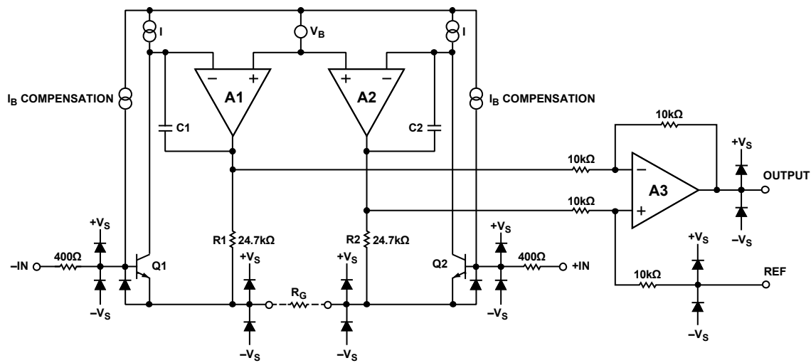
Figure 44. Simplified Schematic
