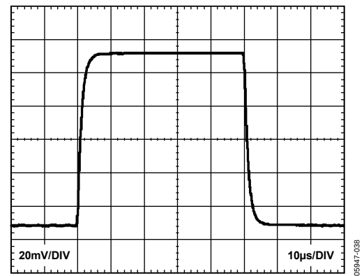
Figure 37. Small Signal Response, G = 100 , R_L = 2 \text{ k}\Omega , C_L = 100 \text{ pF}
