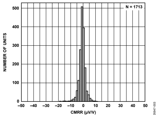
Figure 3. Typical Distribution for CMRR (G = 1)
