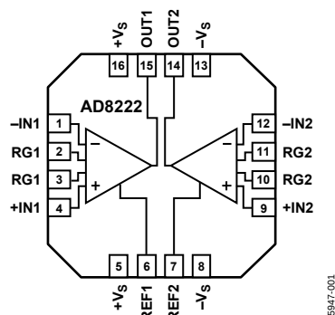
Figure 1. 4 mm × 4 mm LFCSP
