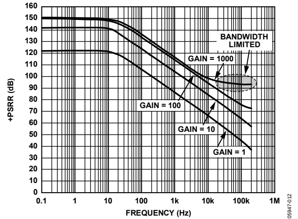
Figure 12. Positive PSRR vs. Frequency, RTI ( G = 1 to 1000)
