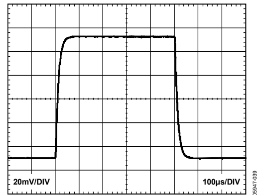
Figure 38. Small Signal Response, G = 1000 , R_L = 2 \text{ k}\Omega , C_L = 100 \text{ pF}
