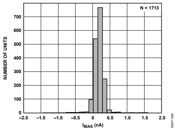
Figure 5. Typical Distribution of Input Bias Current
