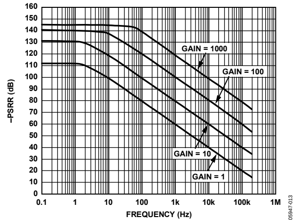
Figure 13. Negative PSRR vs. Frequency, RTI ( G = 1 to 1000)
