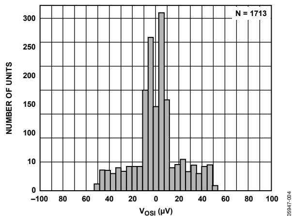
Figure 4. Typical Distribution of Input Offset Voltage
