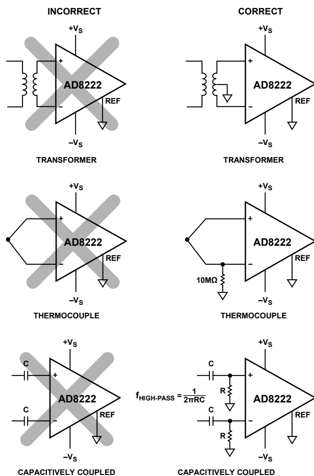
Figure 47. Creating an I_{\text{BIAS}} Path
