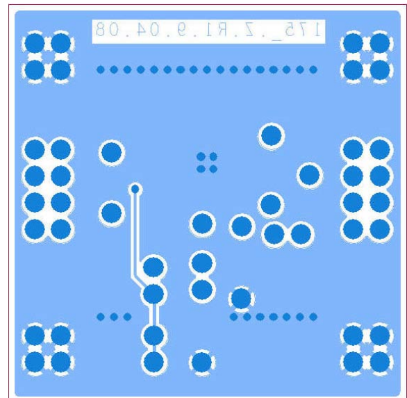
Figure 48. Typical Board Layout—Bottom Side
