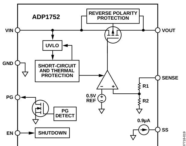
Figure 24. ADP1752 Internal Block Diagram
