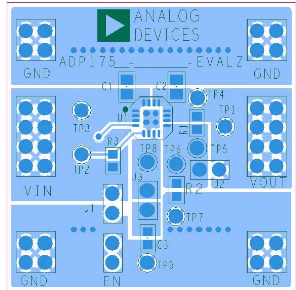
Figure 47. Typical Board Layout—Top Side
