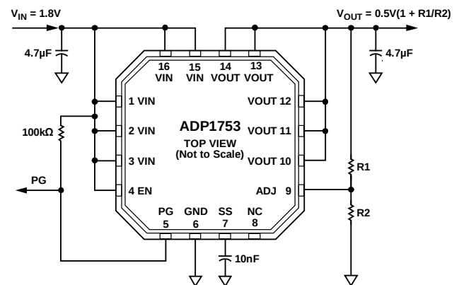
Figure 2. ADP1753 with Adjustable Output Voltage, 0.75 V to 3.0 V
