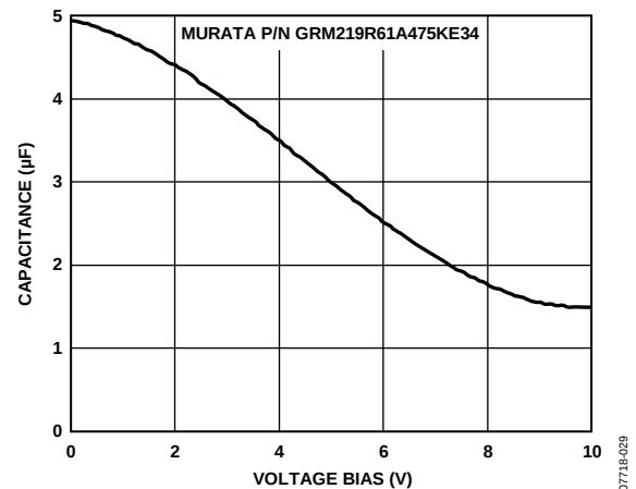
Figure 35. Capacitance vs. Voltage Bias Characteristics
