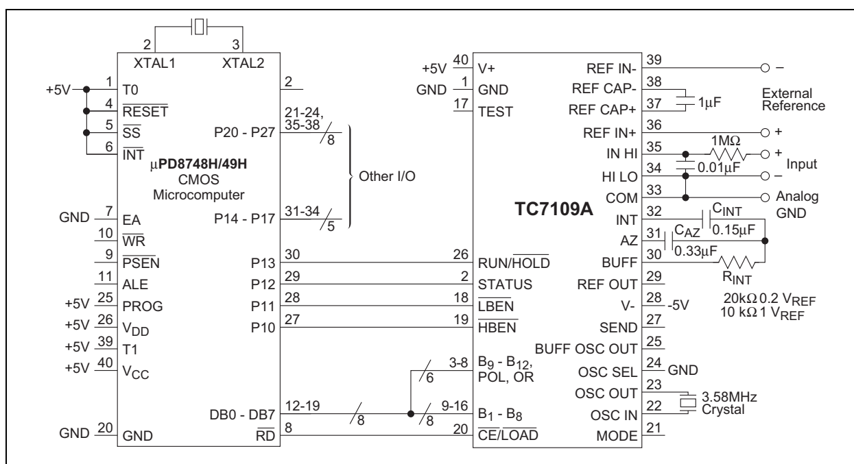
FIGURE 4-8: Connection Diagram
