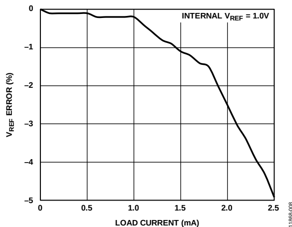
Figure 52. V_{REF} Error (Internal V_{REF} = 1.0 \text{ V} ) vs. Load Current
