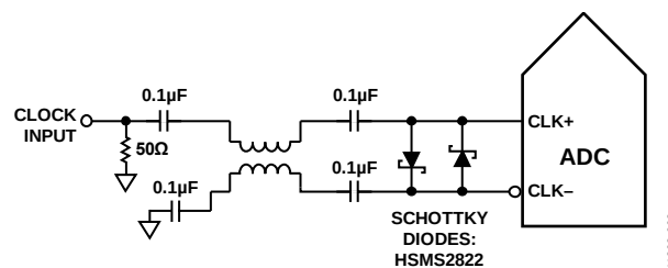
Figure 57. Balun-Coupled Differential Clock (Up to 1 GHz)
