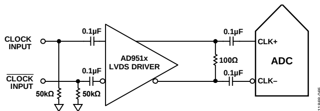
Figure 59. Differential LVDS Sample Clock (Up to 1 GHz)
