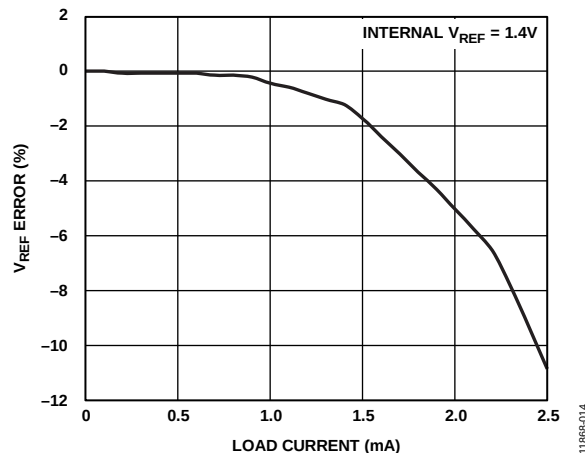
Figure 53. V_{REF} Error (Internal V_{REF} = 1.4 \text{ V} ) vs. Load Current
