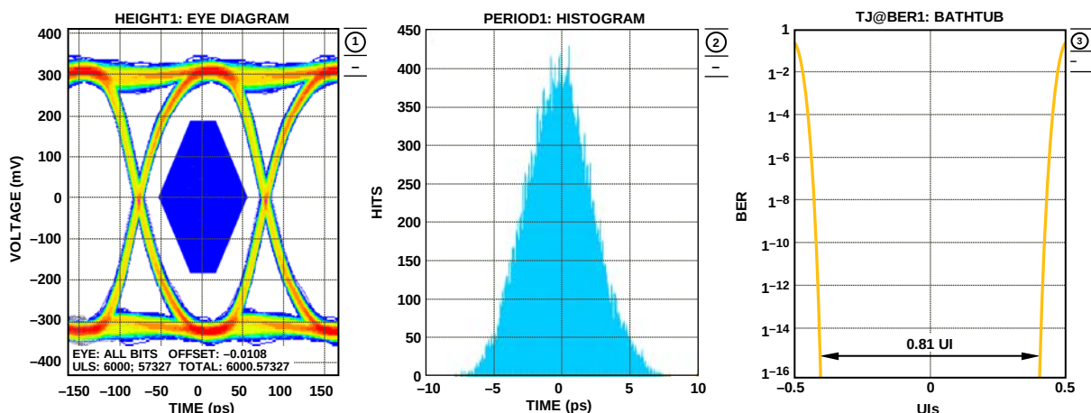
Figure 69. AD9656 Digital Outputs Data Eye, Histogram, and Bathtub, External 100 \Omega Terminations at 6.4 Gbps
