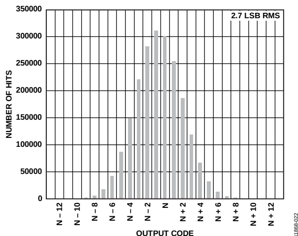
Figure 34. Input Referred Noise Histogram, f_{SAMPLE} = 125 MSPS, V_{REF} = 1.0 V
