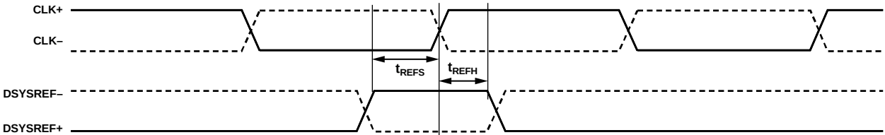
Figure 3. DSYSREF+/DSYSREF- Setup and Hold Timing (Clock Divider = 1)
