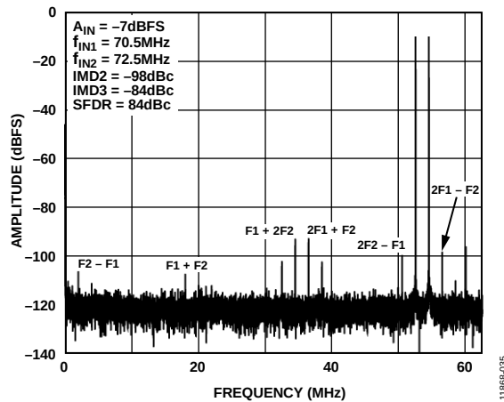
Figure 12. Two-Tone 32k FFT with f_{IN1} = 70.5 MHz and f_{IN2} = 72.5 MHz, f_{SAMPLE} = 125 MSPS, V_{REF} = 1.4 V
