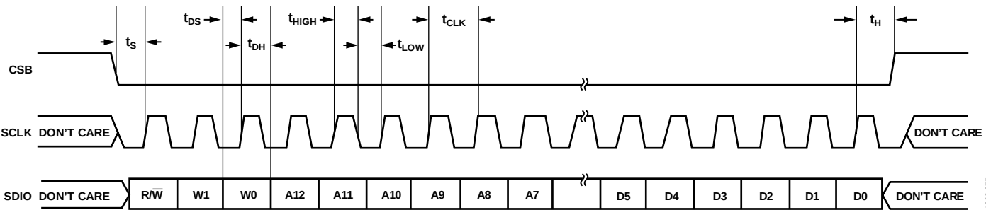
Figure 70. Serial Port Interface Timing Diagram
