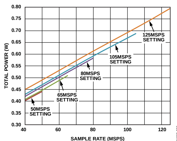
Figure 62. Total Power vs. f_{SAMPLE} for f_{IN} = 9.7 MHz, Four Channels ( V_{REF} = 1.4 V)
