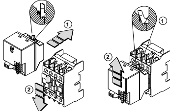
Attaching and removing an LA4SPX to an IEC D-Line Contactor
