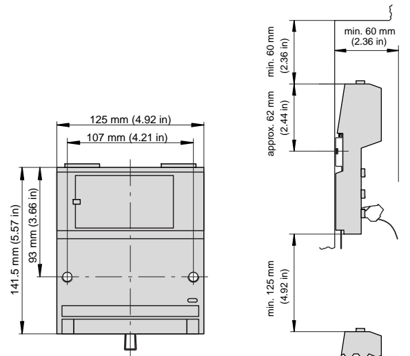
Mounting Hole Locations
