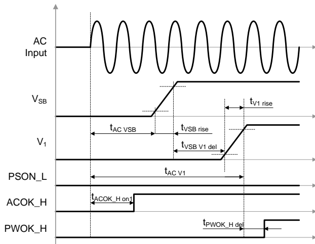
Figure 26: AC turn-on timing
