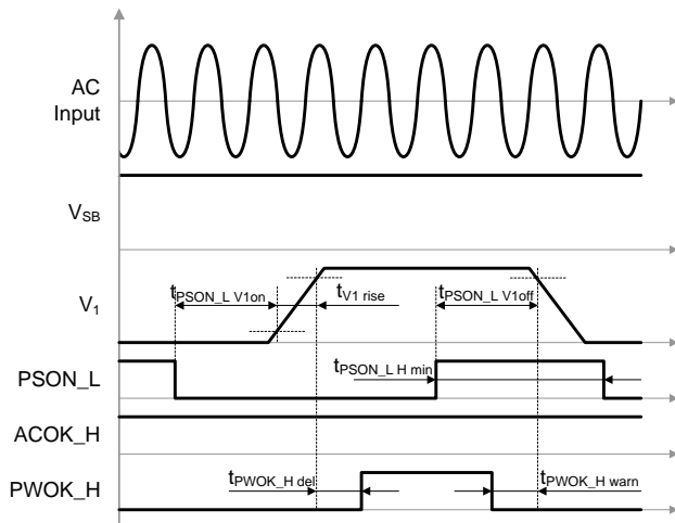
Figure 29: PSON_L turn-on/off timing
