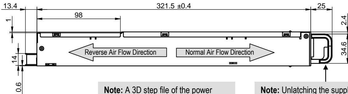
Figure 43: Side view 1
