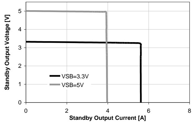
Figure 22: Current limitation on V SB
