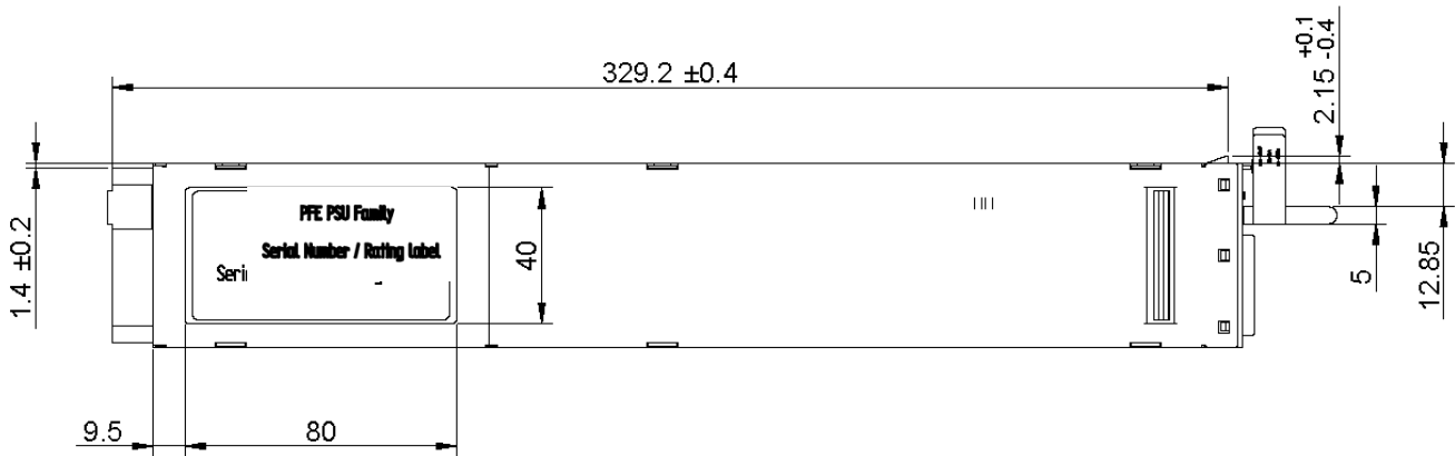
Figure 44: Top view
