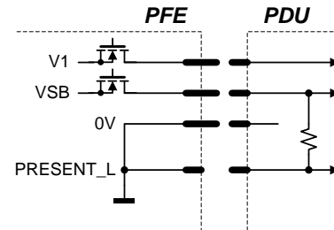
Figure 25: PRESENT_L signal pin
