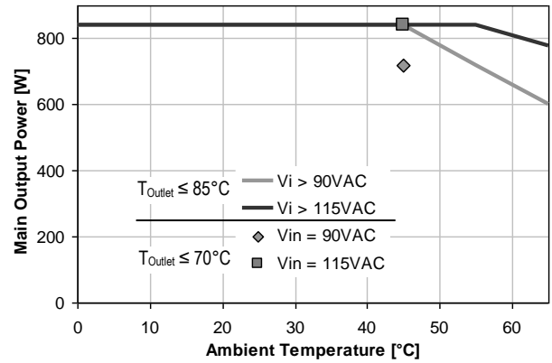
Figure 41: Thermal derating for PFE850-12-054NA
