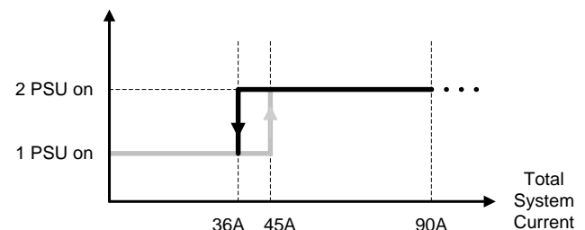
Figure 30: Hot-standby enable/disable current thresholds
