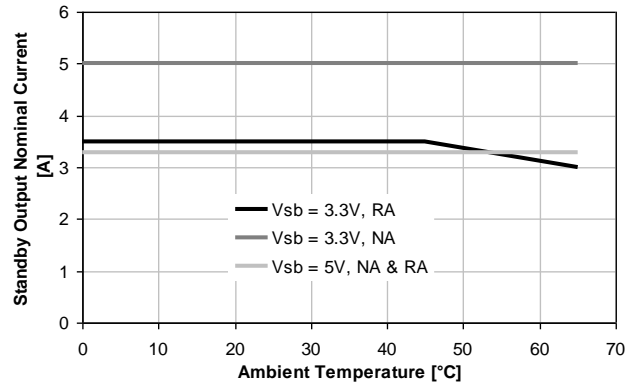
Figure 23: Temperature derating on V SB
