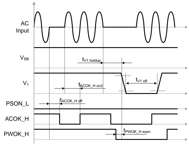
Figure 27: AC short dips
