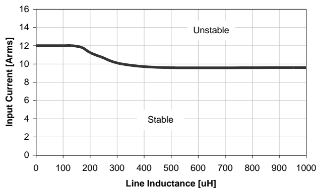
Figure 4: PFC stability region
