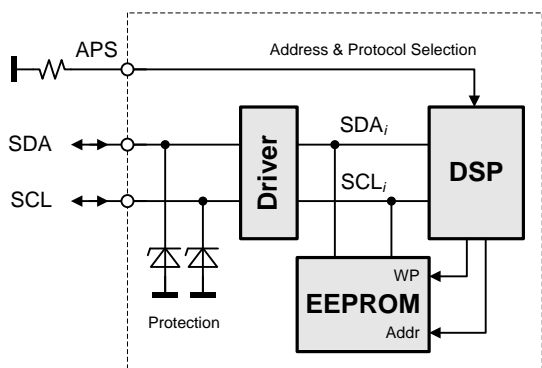
Figure 36: I 2 C Bus to DSP and EEPROM
