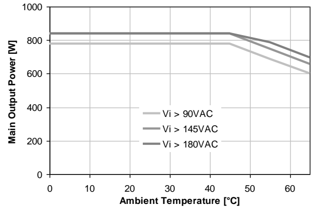
Figure 42: Thermal derating for PFE850-12-054RA
