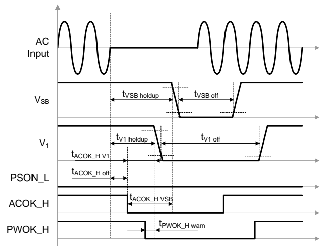
Figure 28: AC long dips
