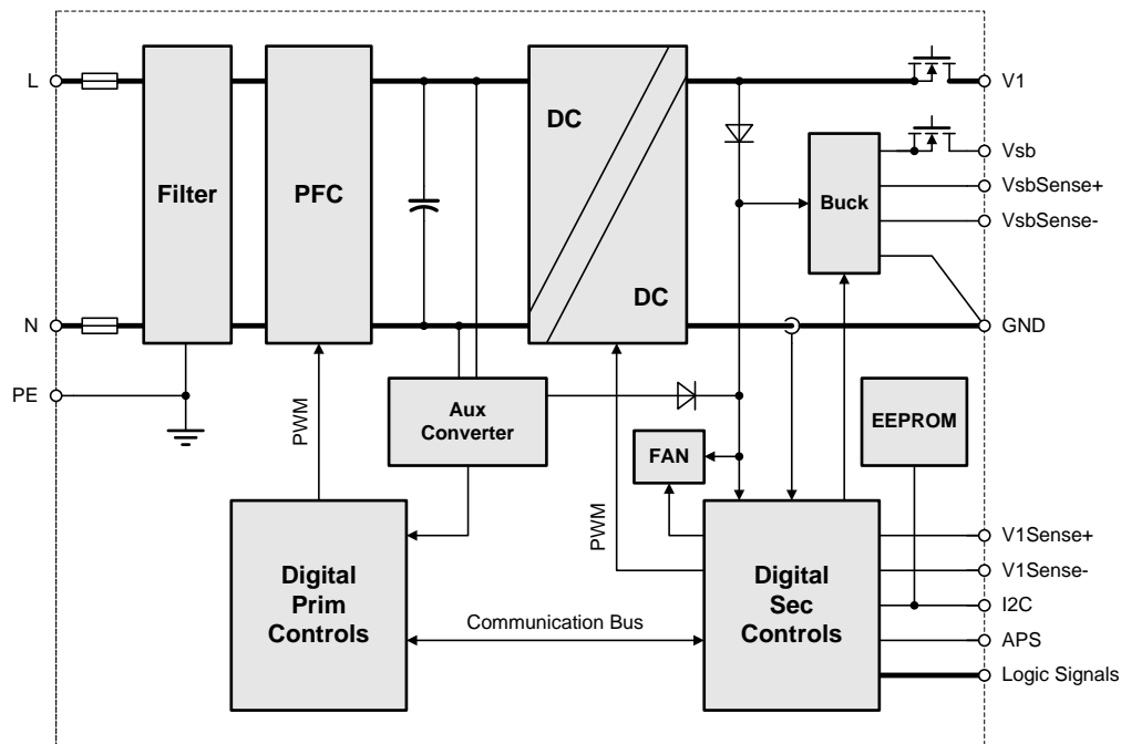
Figure 1: PFE850-12-054xA Block Diagram
