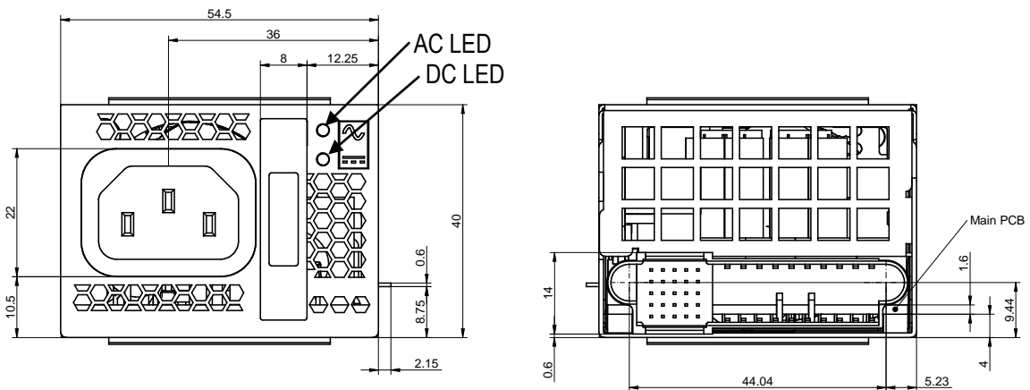
Figure 46: Front view
