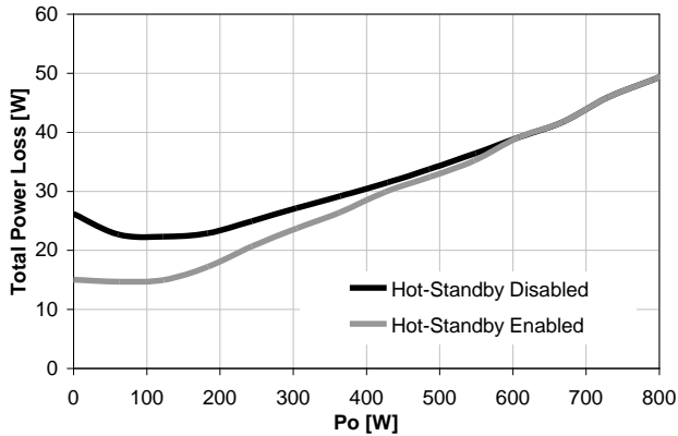
Figure 31: PSU power losses with/without hot-standby mode
