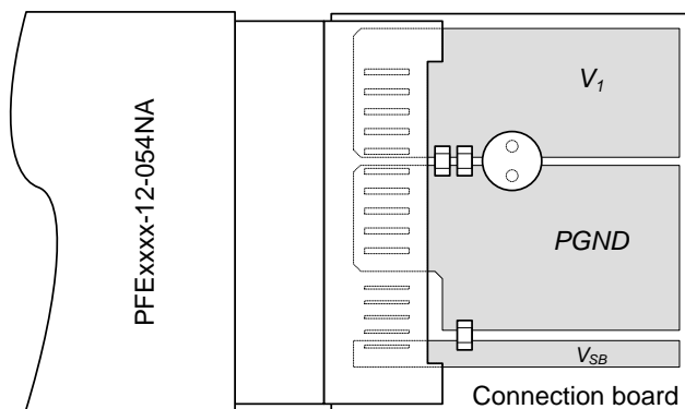
Figure 6: Output ripple test setup
