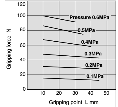
MHSH3-40D
