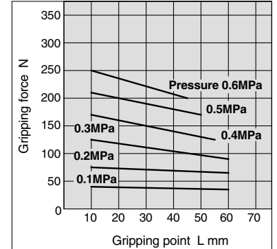
MHSH3-63D
