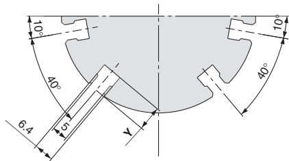
Auto switch mounting groove positions
