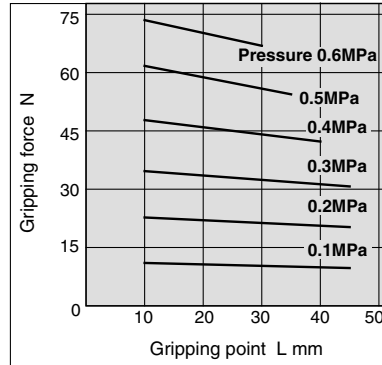
MHS4-40D
