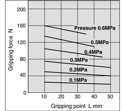
MHSH3-50D
