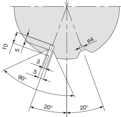
MHSJ3-63D
