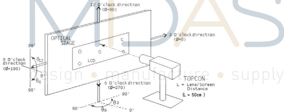
Figure 3. Measurement Set Up
