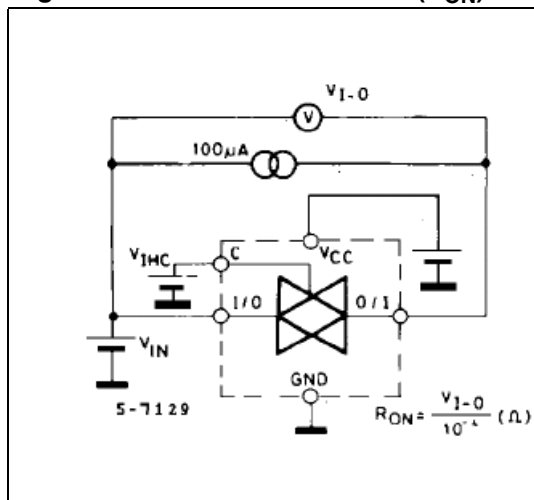
Figure 12. Channel resistance ( R_{ON} )
