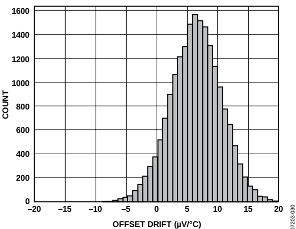
Figure 25. Offset Drift
