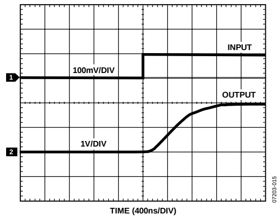
Figure 14. Rise Time
