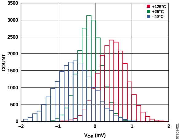
Figure 23. Offset Distribution
