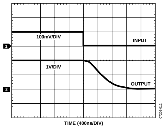
Figure 13. Fall Time
