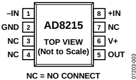
Figure 3. Pin Configuration
