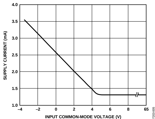
Figure 12. Supply Current vs. Common-Mode Voltage
