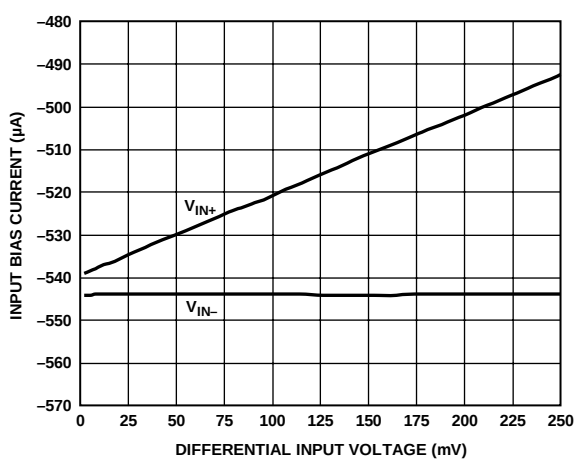
Figure 9. Input Bias Current vs. Differential Input Voltage, V_{CM} = 0 \text{ V}
