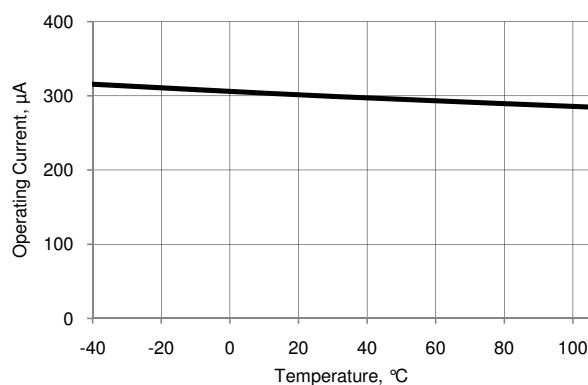
Figure 11-68. VDAC Operating Current vs Temperature, 1 V Mode, Fast Mode
