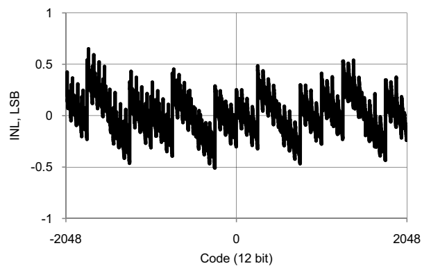
Figure 11-42. SAR ADC INL vs Output Code, Bypassed Internal Reference Mode
