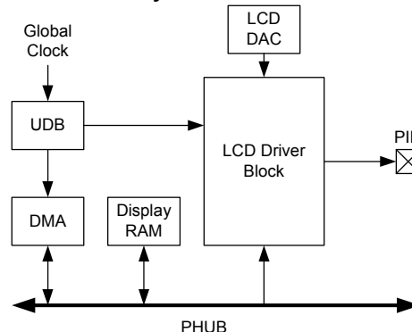
Figure 8-11. LCD System
