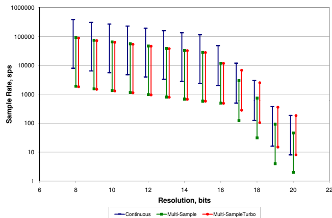
Figure 8-3. Delta-sigma ADC Sample Rates, Range = \pm 1.024 V
