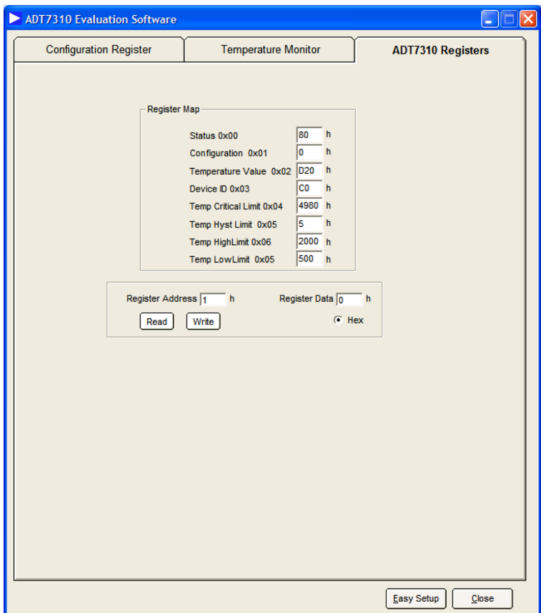
Figure 8. ADT7310 Registers
