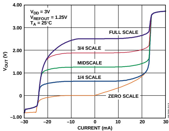
Figure 20. Source and Sink Current Capability with V_{DD} = 3\text{ V}
