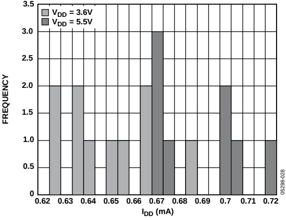
Figure 16. I_{DD} Histogram with External Reference
