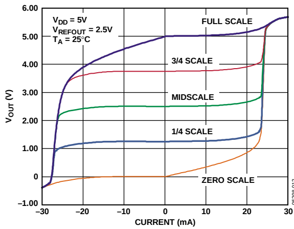
Figure 19. Source and Sink Current Capability with V_{DD} = 5\text{ V}
