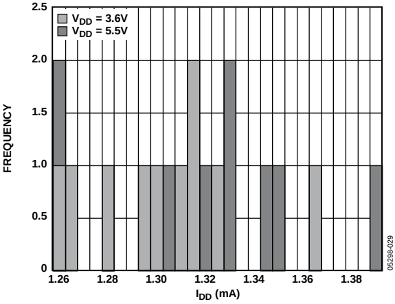
Figure 17. I_{DD} Histogram with Internal Reference
