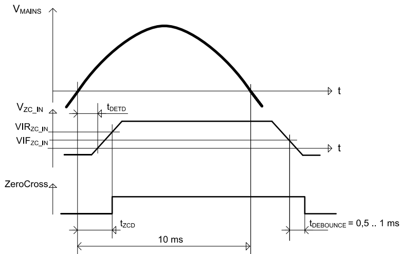
Figure 13. Zero Cross Detector Signals and Timing (example for 50 Hz)
