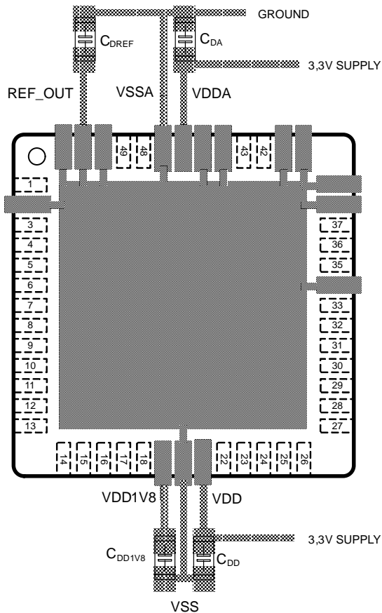
Figure 28. Recommended Layout of the Placement of Decoupling Capacitors (bottom ground plane not shown)
