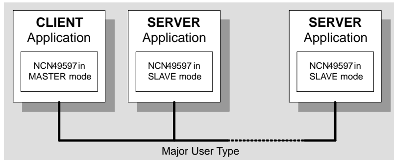
Figure 8. Application Example: a Network Topology for a Three-node IEC 61334-5-1 Network
