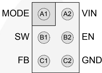
Figure 2. WLCSP, Bumps Facing Down
