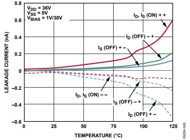
Figure 16. Leakage Currents vs. Temperature, 36 V Single Supply
