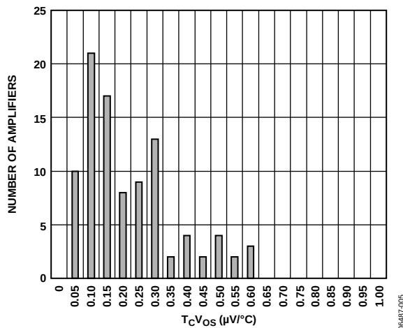
Figure 5. T_CV_{OS} Distribution
