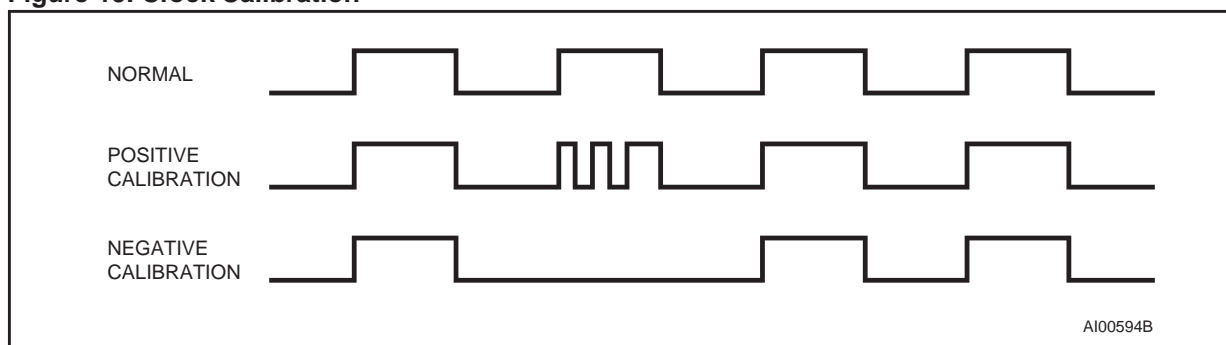
Figure 19. Clock Calibration
