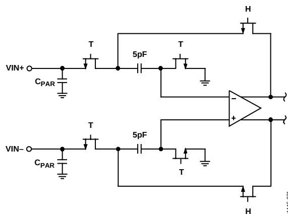
Figure 31. Switched-Capacitor Input
