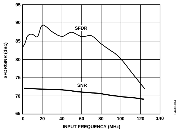
Figure 14. AD9248-40 Single-Tone SFDR/SNR vs. f_{IN}
