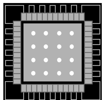
Figure 58. Thermal Via Array
