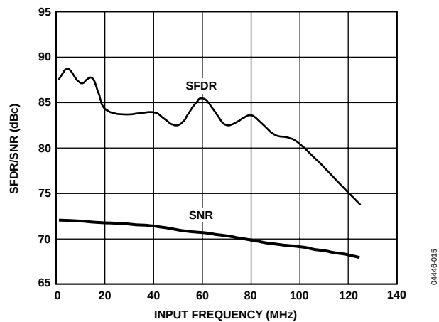
Figure 15. AD9248-20 Single-Tone SFDR/SNR vs. f_{IN}
