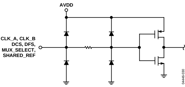
Figure 30. Equivalent Digital Input Circuit
