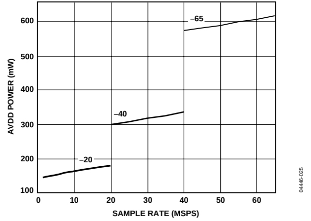
Figure 25. Analog Power Consumption vs. FS
