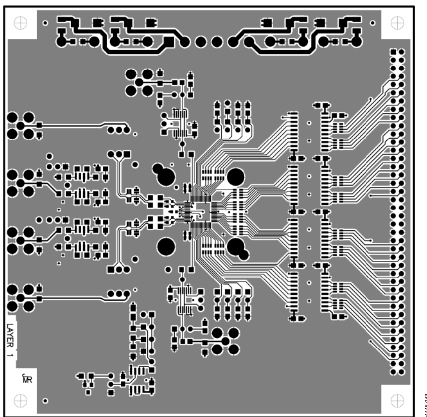
Figure 43. PCB Top Layer
