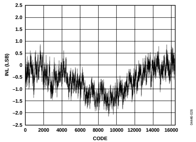
Figure 26. AD9248-65 Typical INL
