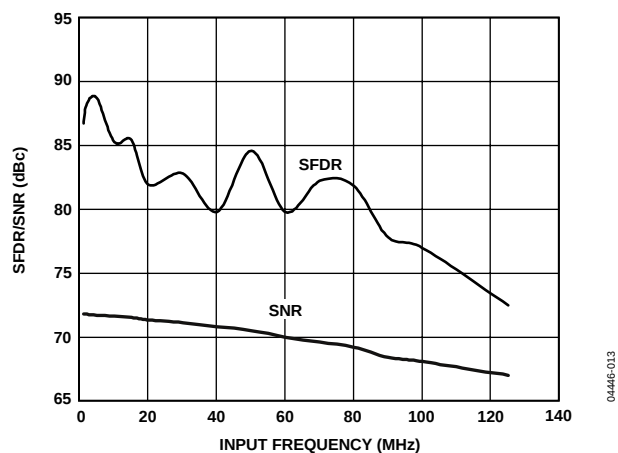
Figure 13. AD9248-65 Single-Tone SFDR/SNR vs. f_{IN}
