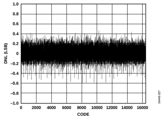
Figure 27. AD9248-65 Typical DNL
