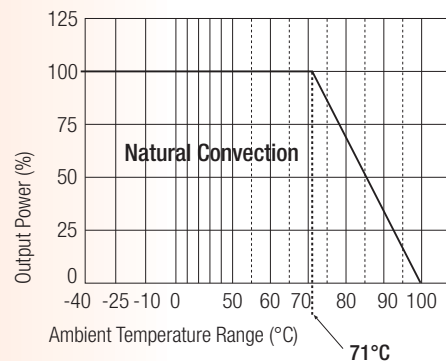
RP20-2412DEW With Heat Sink
