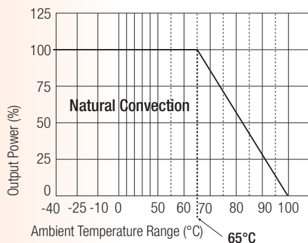
RP20-2412SEW With Heat Sink
