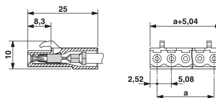
Dimensioned drawing
