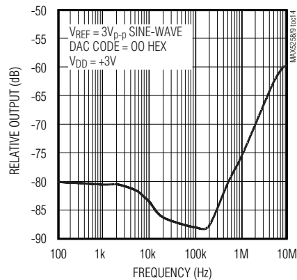
REFERENCE FEEDTHROUGH vs. FREQUENCY
