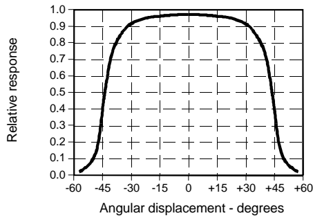
Fig. 1 Responsivity vs Angular Displacement (SD3410)
