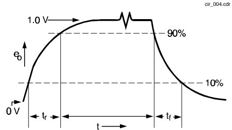
SWITCHING WAVEFORM
