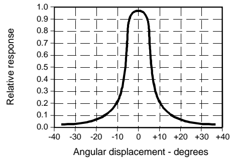
Fig. 2 Responsivity vs Angular Displacement (SD5410)
