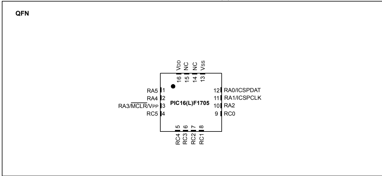
FIGURE 2: 16-PIN PACKAGE DIAGRAM FOR PIC16(L)F1705
