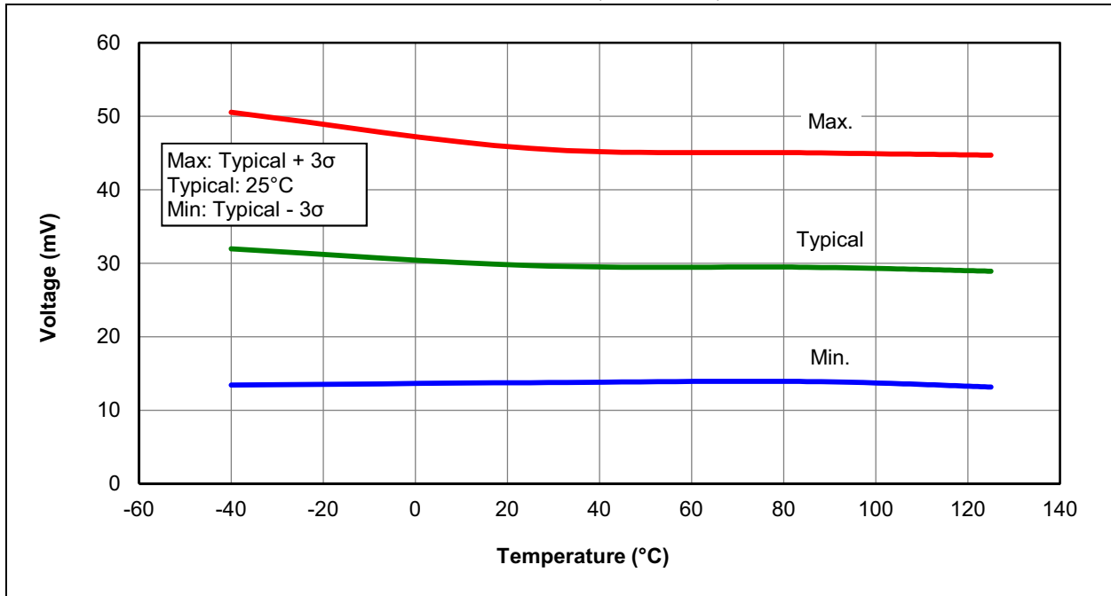
FIGURE 33-10: BROWN-OUT RESET HYSTERESIS, BORV = 1, PIC16LF1705/9 ONLY
