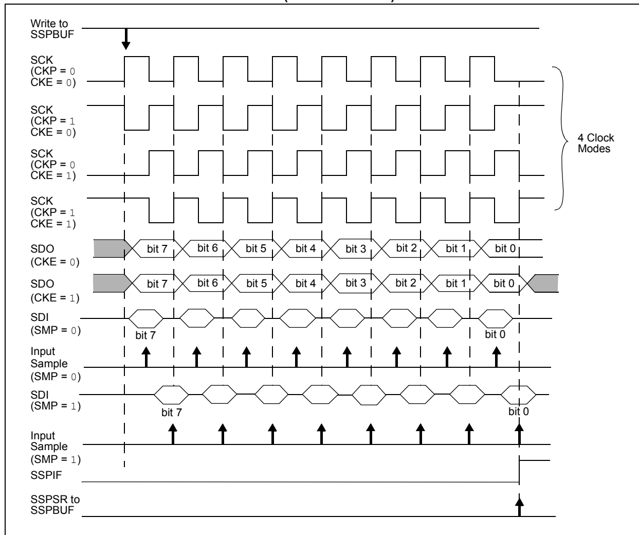
FIGURE 28-6: SPI MODE WAVEFORM (MASTER MODE)
