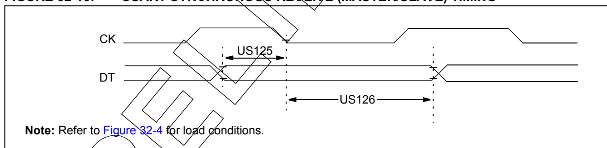
FIGURE 32-16: USART SYNCHRONOUS RECEIVE (MASTER/SLAVE) TIMING
