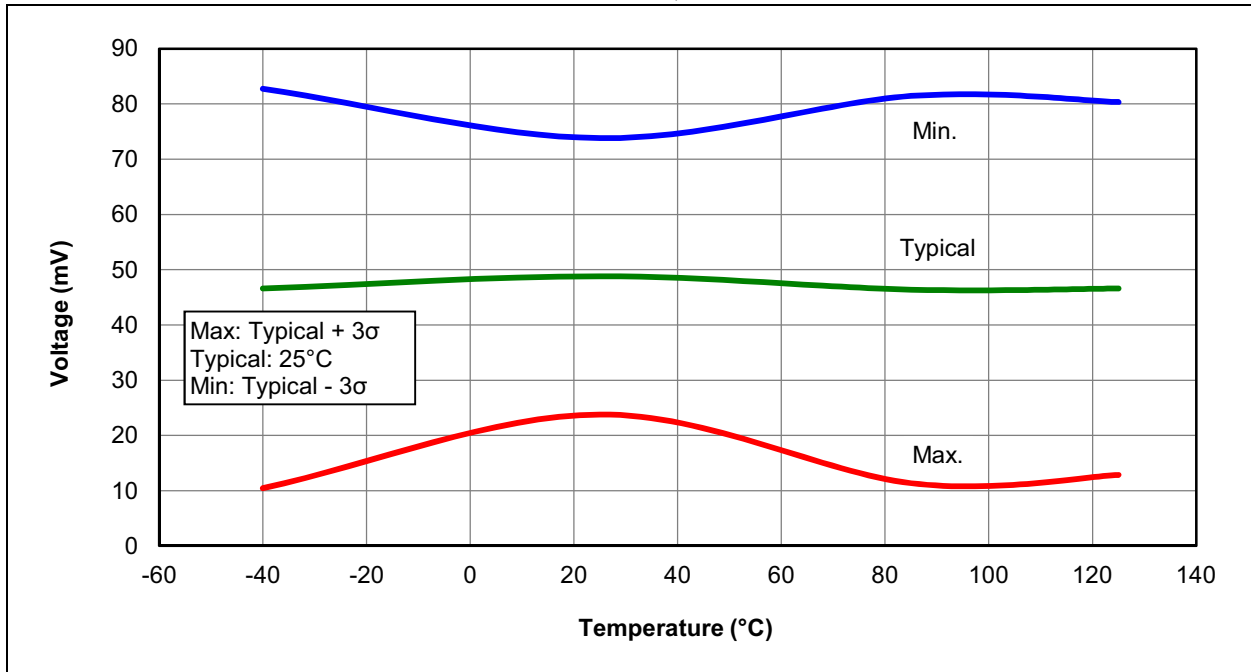
FIGURE 33-14: BROWN-OUT RESET HYSTERESIS, BORV = 0
