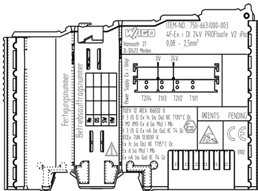
Figure 9: Side marking example for approved Ex i I/O modules according to ATEX and IECEx.
