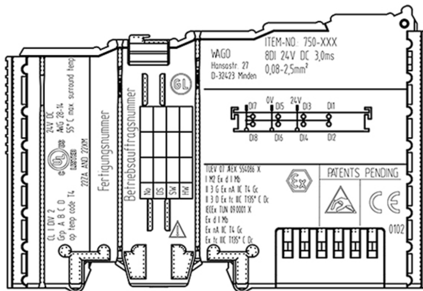
Figure 7: Side marking example for approved I/O modules according to ATEX and IECEx
