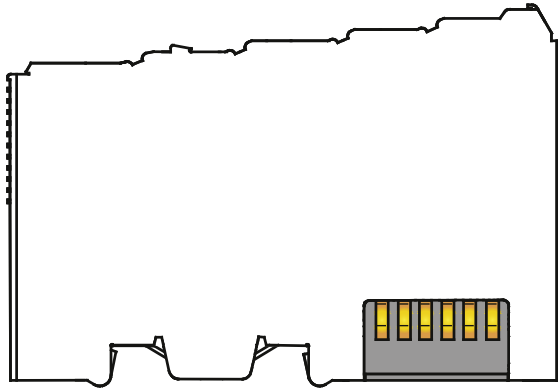
Figure 6: Data contacts
