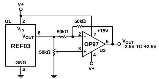
Figure 44. Negatively Adjustable Reference
