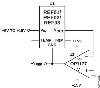
Figure 39. Negative Reference
