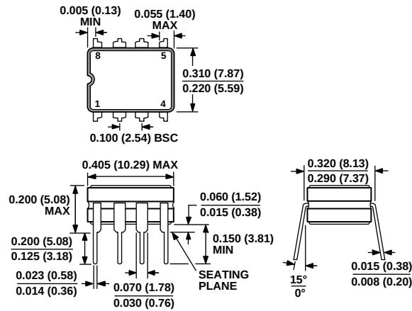
Figure 45. 8-Lead Ceramic Dual In-Line Package [CERDIP]
