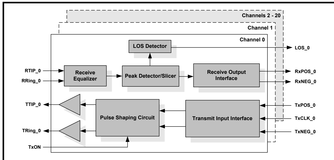
FIGURE 1. BLOCK DIAGRAM OF THE XRT59L921
