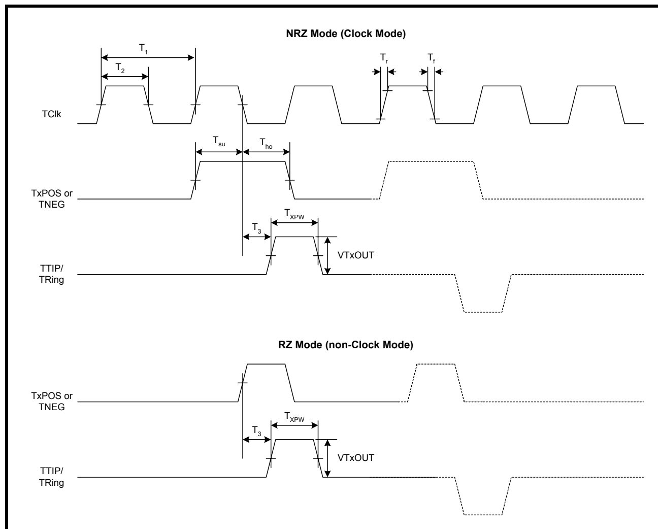
FIGURE 15. TRANSMIT TIMING DIAGRAM
