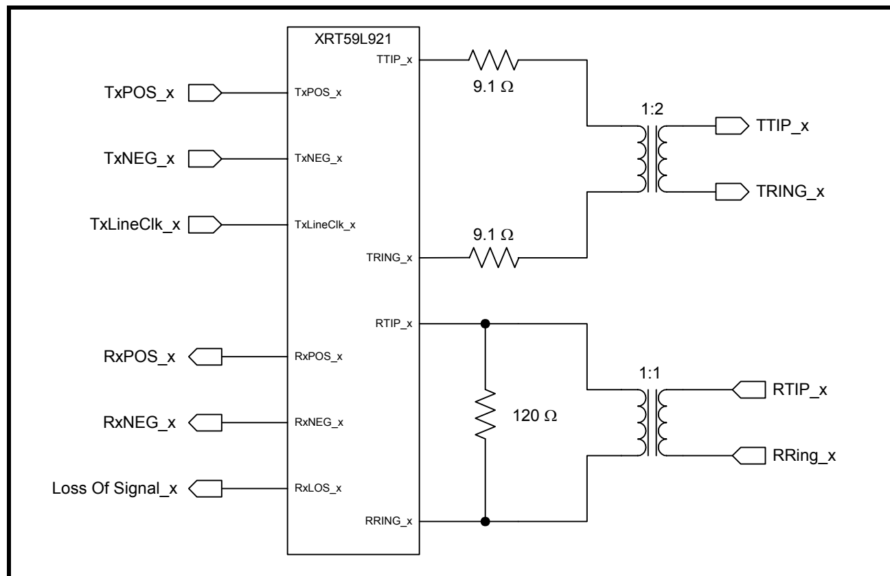
FIGURE 18. ILLUSTRATION ON HOW TO INTERFACE CHANNEL 1 (OF THE XRT59L921) TO THE LINE (RECEIVER IS TRANSFORMER-COUPLED TO A 120\Omega BALANCED LINE)
