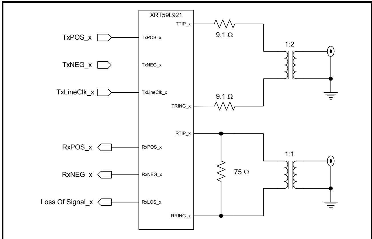
FIGURE 17. ILLUSTRATION ON HOW TO INTERFACE CHANNEL 1 (OF THE XRT59L921) TO THE LINE (RECEIVER IS TRANSFORMER-COUPLED TO A 75\Omega UNBALANCED LINE)
